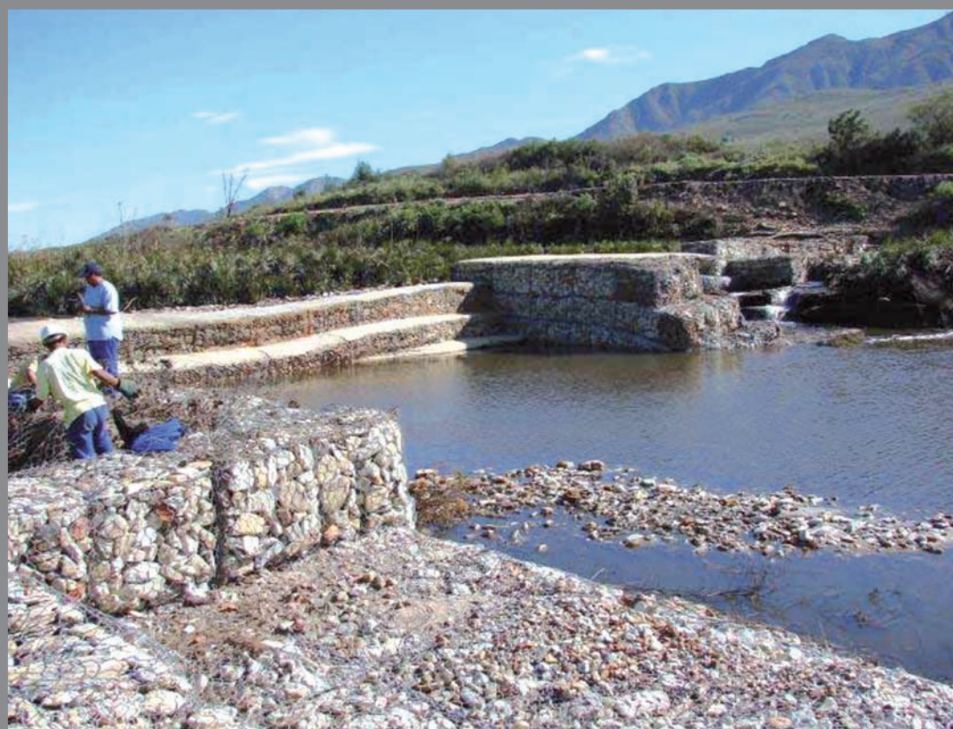
Figure 11: Top: Gabion C at Hudsonvale in 2002.
