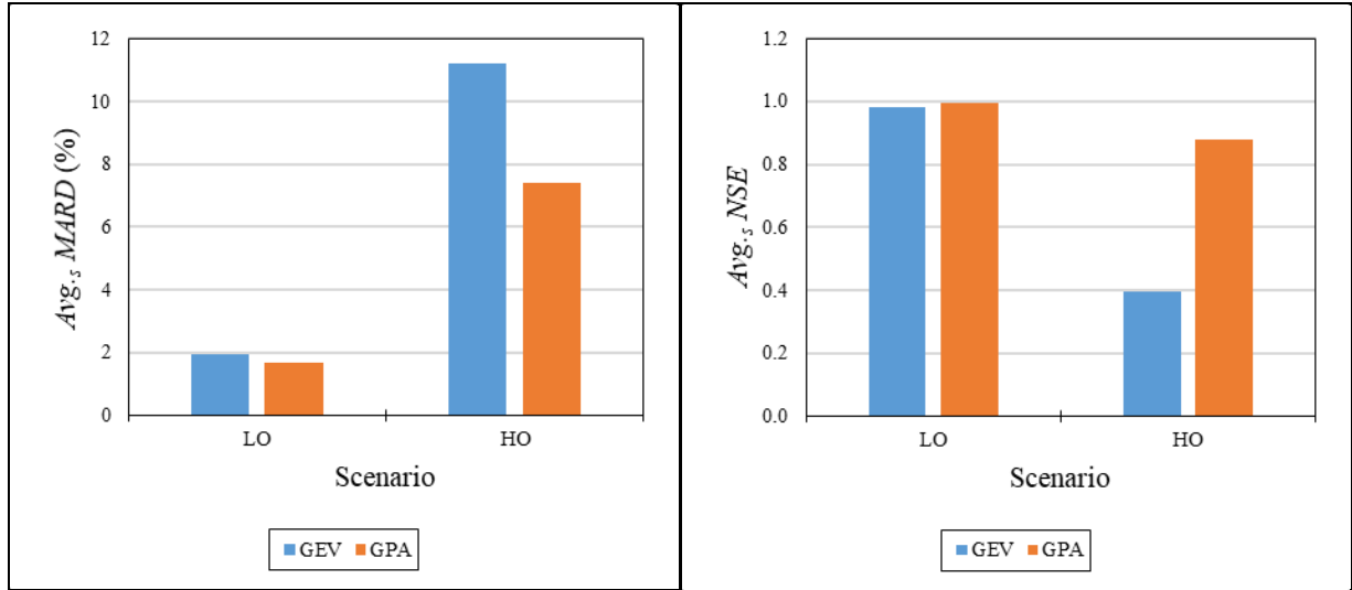
Figure 3.19 Avg.s MARD and Avg.s NSE for design rainfall events estimated using synthetically generated data with LOs and HOs
