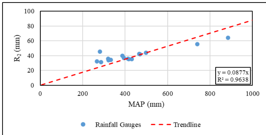
Figure 3.42 R_2 vs MAP for the NI homogenous region
