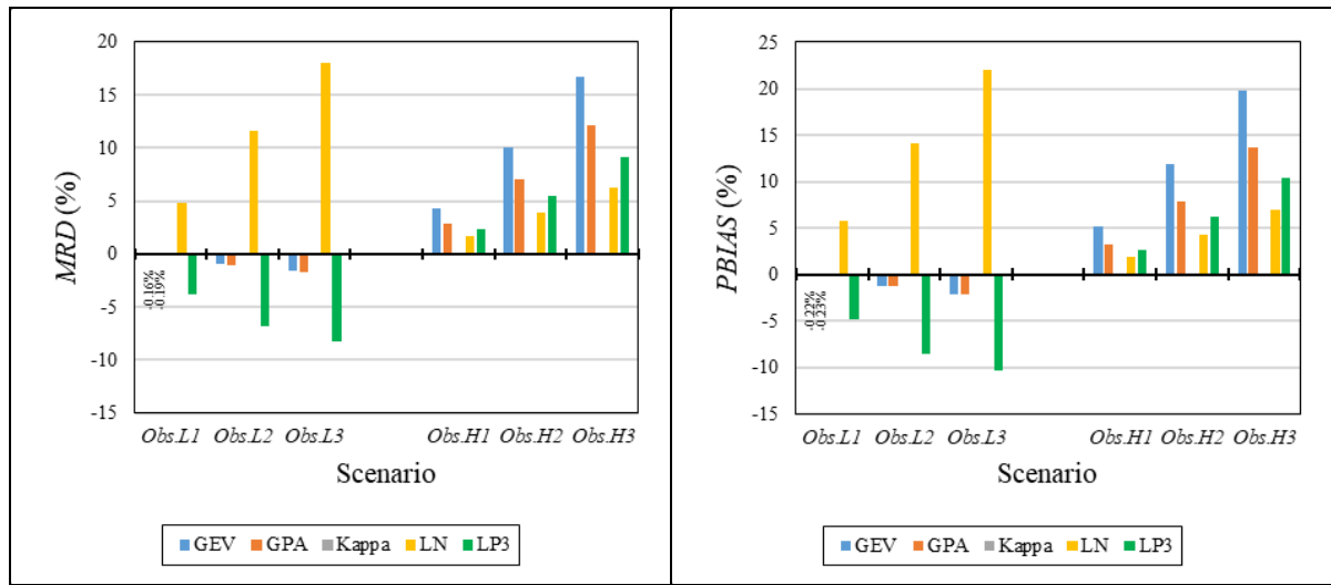
Figure 3.10 MRD and PBIAS for design rainfall events estimated using observed data for Rain Gauge 0042227 for LO (Obs.L1, Obs.L2 and Obs.L3) and HO (Obs.H1, Obs.H2 and Obs.H3) scenarios
