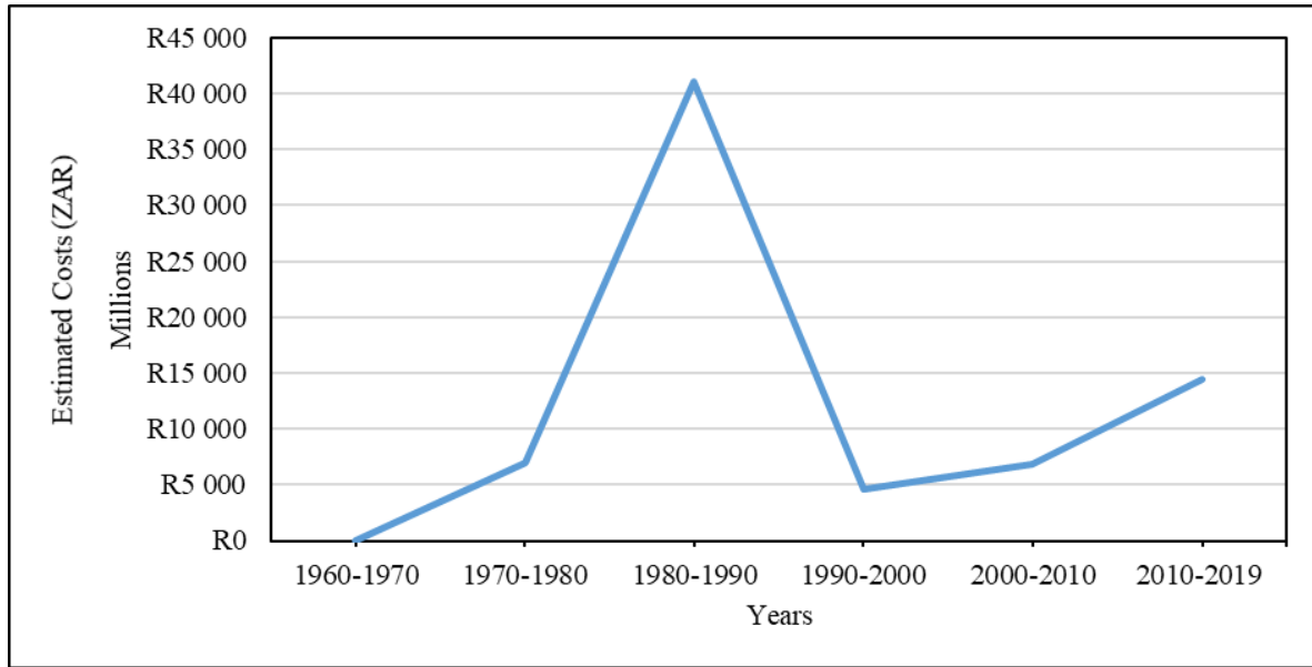
Figure 2.9 Reported estimated costs for regional floods in South Africa
