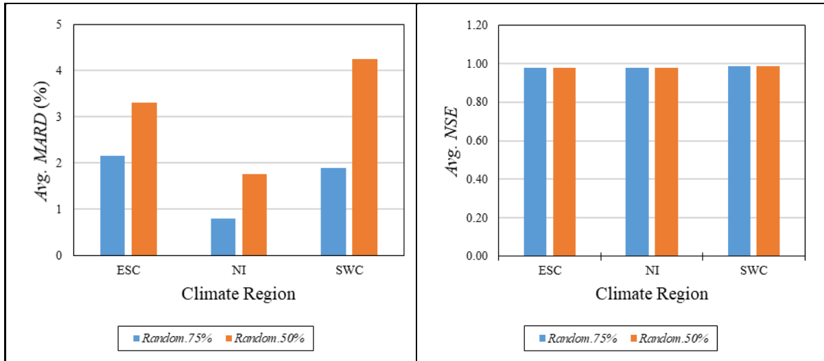
Figure 3.50 Avg. MARD and Avg. NSE of design rainfall events computed using a 75% and 50% randomly reduced gauge network
