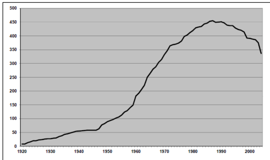
Figure 3.4 Number of useful streamflow gauges open in each year in South Africa (Pitman, 2011)
