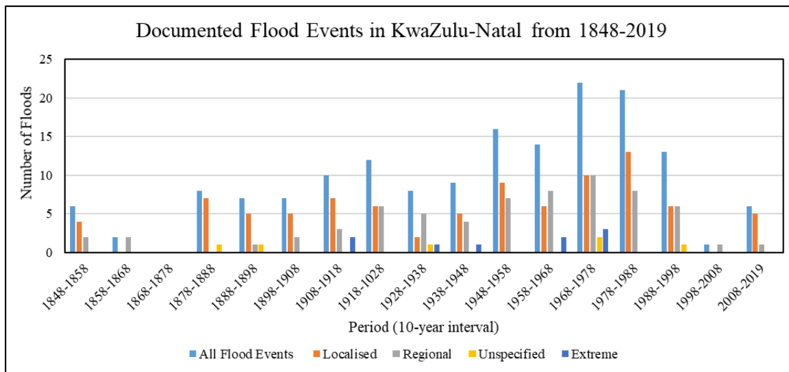
Figure 2.6 Number of documented flood events in KwaZulu-Natal from 1848-2019 illustrates a time series of flood events for KwaZulu-Natal. Typically, there are more localised events than regional events documented in the province.
