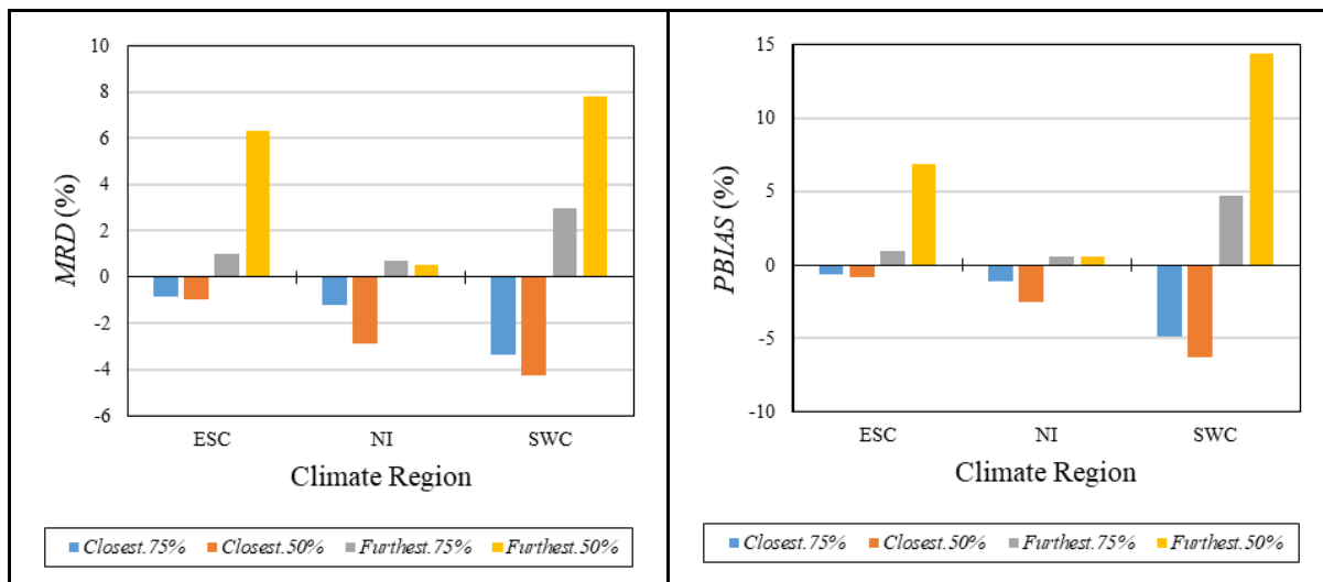
Figure 3.43 MRD and PBIAS for design rainfall events estimated using scenarios ( Closest.75% , Closest.50% , Furthest.75% and Furthest.50% ) of a systematically reduced gauge network
