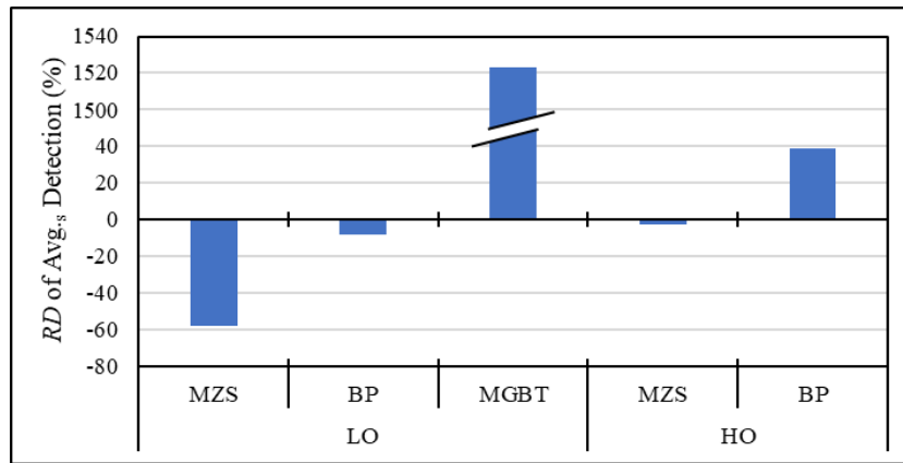
Figure 3.29 RD of Avg. Detection of LOs and HOs in synthetically generated streamflow data series using the BP, MZS and MGBT
