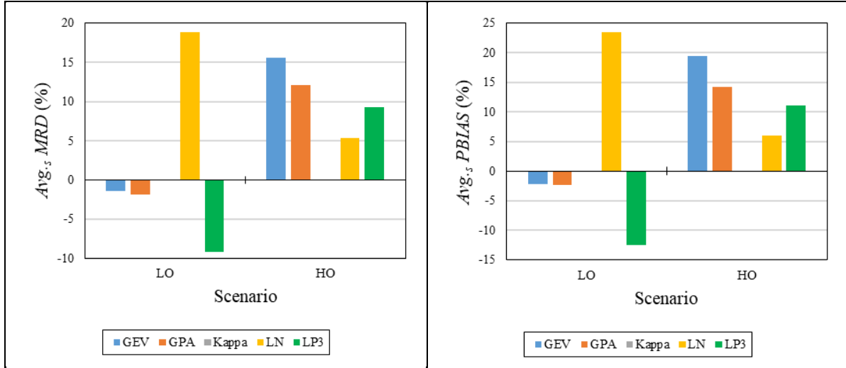
Figure 3.12 Avg.s\ MRD and Avg.s\ PBIAS for design rainfall events estimated using observed data with LOs and HOs
