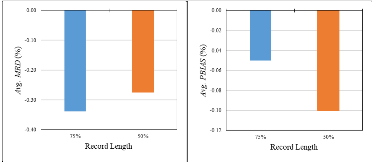
Figure 3.35 Avg. MRD and Avg. PBIAS for design rainfall events estimated using 75% and 50% of AMS records
