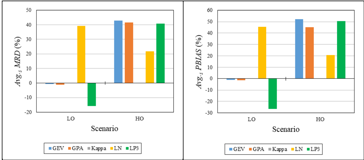
Figure 3.14 Avg.s MRD and Avg.s PBIAS between design flood events estimated using observed data with LOs and HOs
