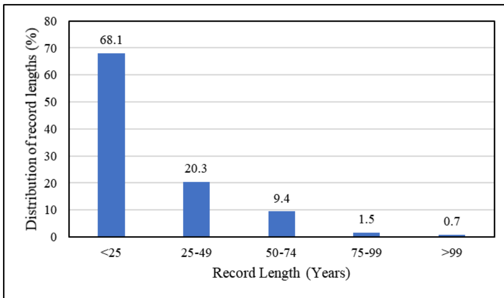
Figure 3.3 Distribution of record lengths in the long duration rainfall database for Southern Africa (after Smithers and Schulze, 2000b)
