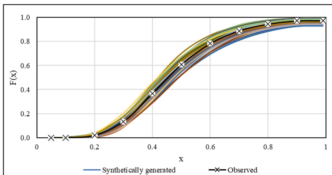
Figure 3.17 CDF for the observed and 100 synthetically generated rainfall data series at Rain Gauge 0268640
