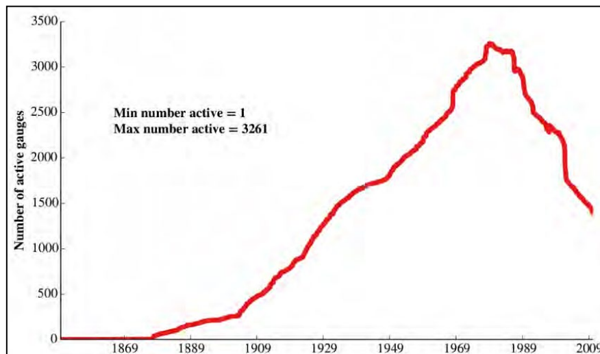
Figure 3.1 Annual active daily rainfall gauges in each year from the daily rainfall database maintained by CSAG (Pegram et al. , 2016)
