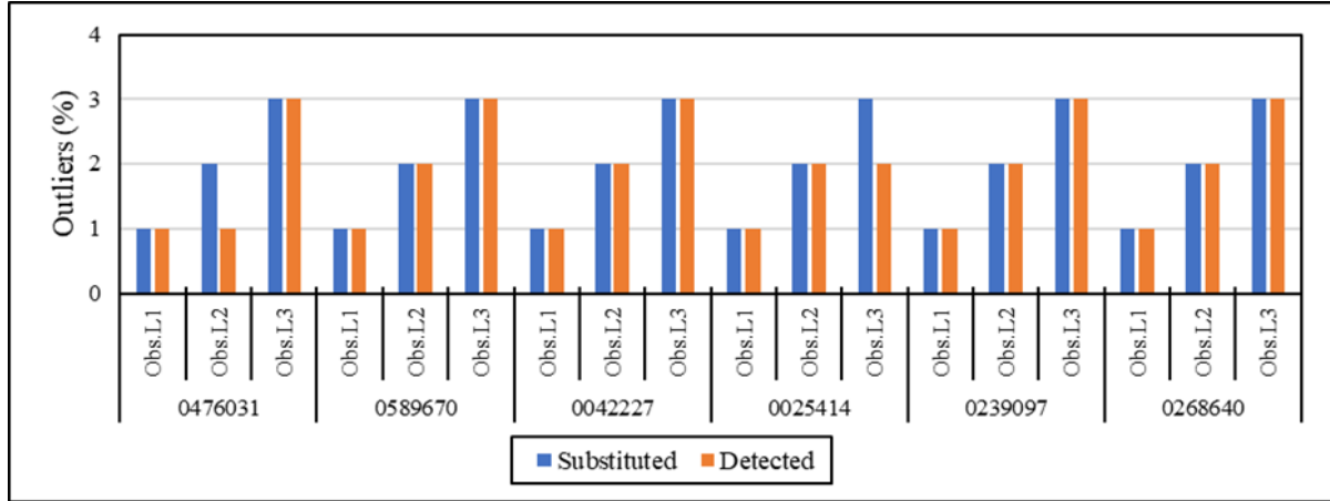
Figure 3.25 Percentage of substituted and detected outliers using the MGBT on observed rainfall data with LO (Obs.L1, Obs.L2 and Obs.L3) scenarios
