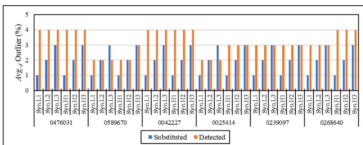
Figure C.4 Percentage of substituted and detected outliers using the BP method on synthetically generated rainfall data series with LO ( Syn.L1 , Syn.L2 and Syn.L3 ) and HO ( Syn.H1 , Syn.H2 and Syn.H3 ) scenarios
