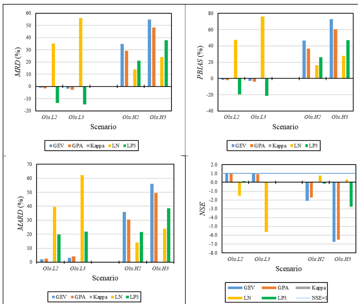
Figure B1.11 Impact of LO ( Obs.L2 and Obs.L3 ) and HO ( Obs.H2 and Obs.H3 ) scenarios on design floods estimated by different PDs from observed data in Catchment V2H004
