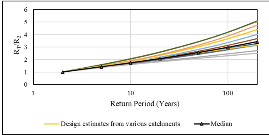
Figure 3.41 Growth curve for design rainfall in Region NI
