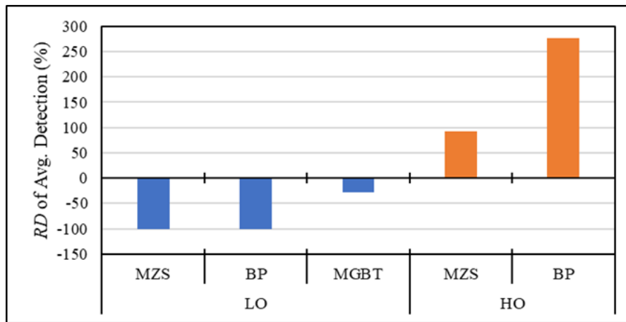
Figure 3.27 RD of Avg. Detection of LOs and HOs in observed streamflow data using the BP, MZS and MGBT
