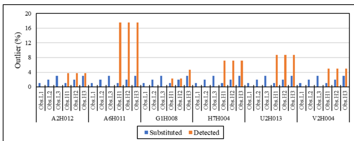
Figure C.1 Percentage of substituted and detected outliers using the BP method on observed streamflow data with LO ( Obs.L1 , Obs.L2 and Obs.L3 ) and HO ( Obs.H1 , Obs.H2 and Obs.H3 ) scenarios
