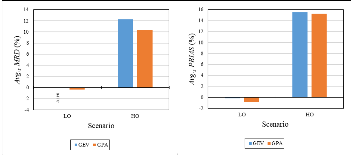
Figure 3.20 Avg.s\ MRD and Avg.s\ PBIAS for design flood events estimated using synthetically generated data with LOs and HOs
