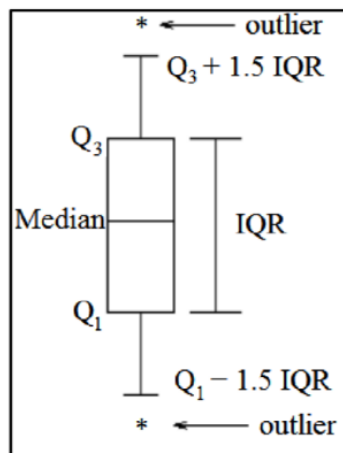
Figure 3.6 Classification of an outlier using the BoxPlot method (Asikoglu, 2017)
