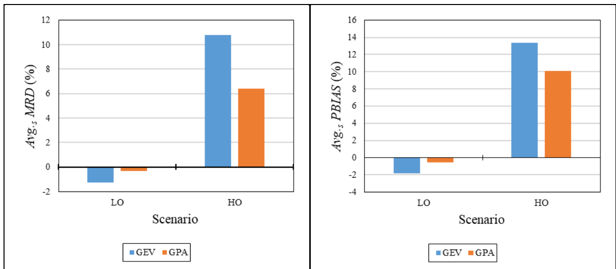
Figure 3.18 Avg.s MRD and Avg.s PBIAS for design rainfall events estimated using synthetically generated data with LOs and HOs
