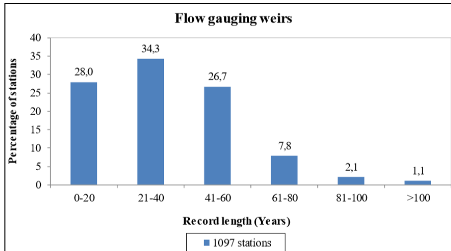
Figure 3.5 Distribution of record lengths for all flow gauging weirs across South Africa (Nathanael, 2015)
