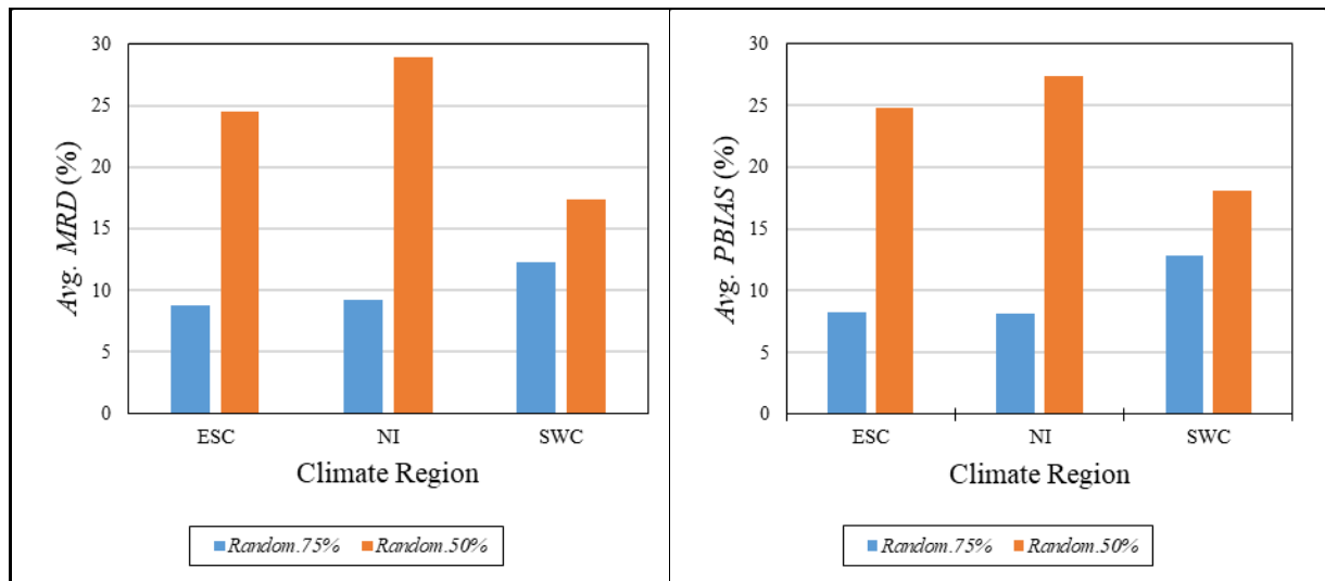
Figure 3.51 Avg. MRD and Avg. PBIAS of design flood events computed using a 75% and 50% randomly reduced gauge network
