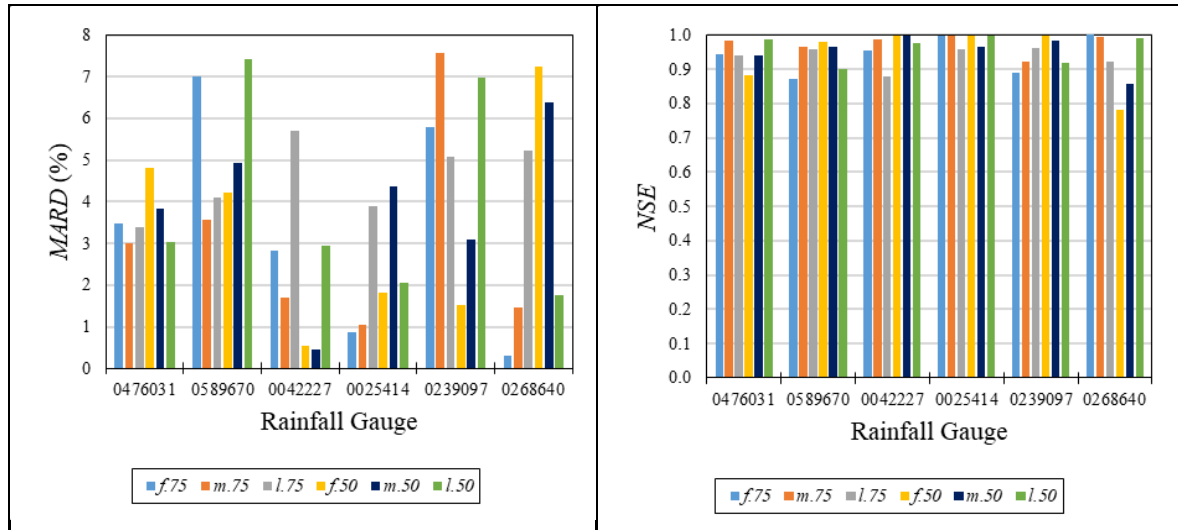
Figure 3.32 MARD and NSE for design rainfall events estimated using scenarios of 75% (f.75, m.75, l.75) and 50% (f.50, m.50, l.50) of record length
