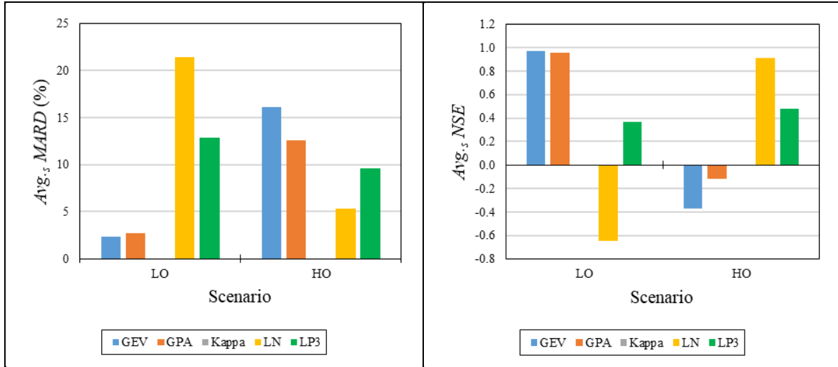
Figure 3.13 Avg.s MARD and Avg.s NSE for design rainfall events estimated using observed data with LOs and HOs
