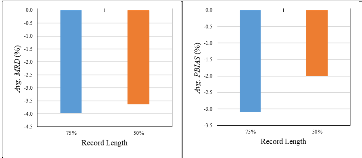
Figure 3.37 Avg. MRD and Avg. PBIAS for design flood events estimated using 75% and 50% of AMS records
