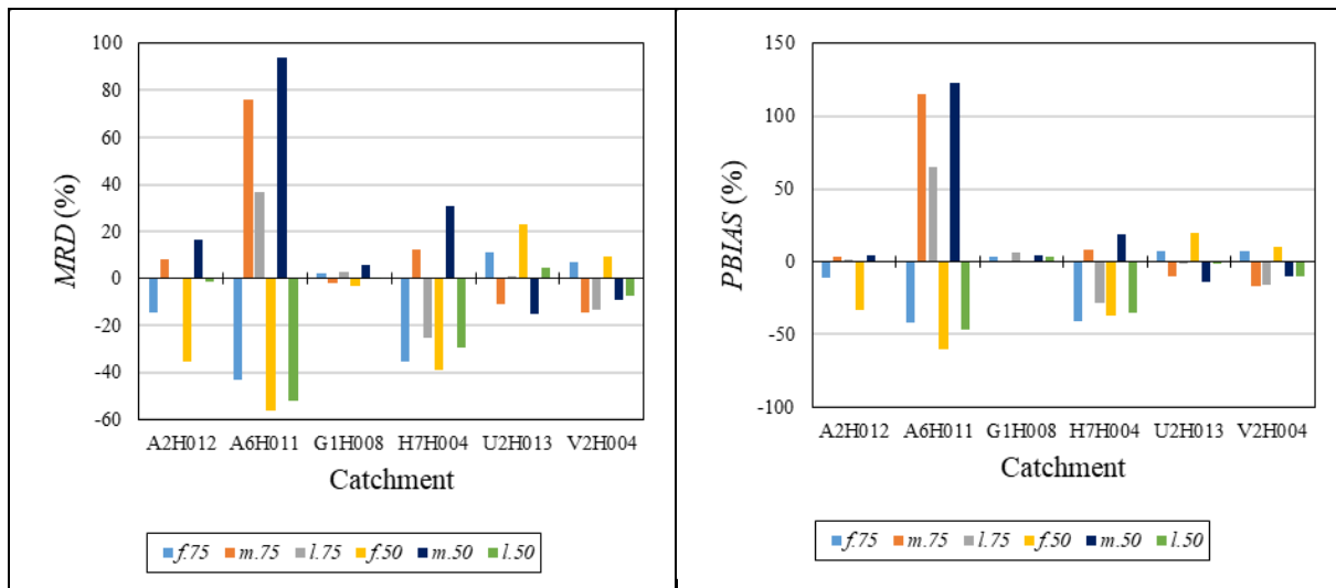
Figure 3.33 MRD and PBIAS for design flood events estimated using scenarios of 75% (f.75, m.75, l.75) and 50% (f.50, m.50, l.50) of record length
