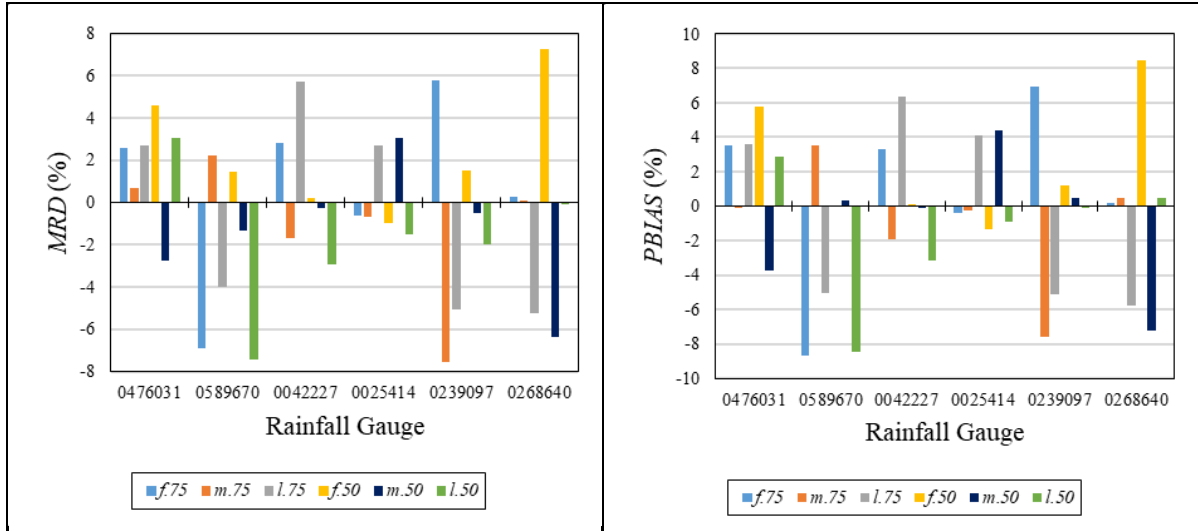
Figure 3.31 MRD and PBIAS for design rainfall events estimated using scenarios of 75% (f.75, m.75, l.75) and 50% (f.50, m.50, l.50) of record length
