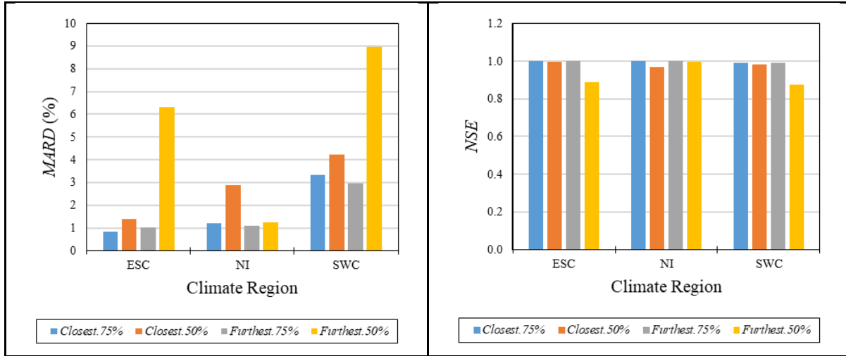
Figure 3.44 MARD and NSE for design rainfall events estimated using scenarios (Closest.75%, Closest.50%, Furthest.75% and Furthest.50%) of a systematically reduced gauge network
