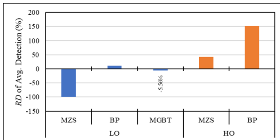
Figure 3.26 RD of Avg. Detection of LOs and HOs in observed rainfall data using the BP, MZS and MGBT
