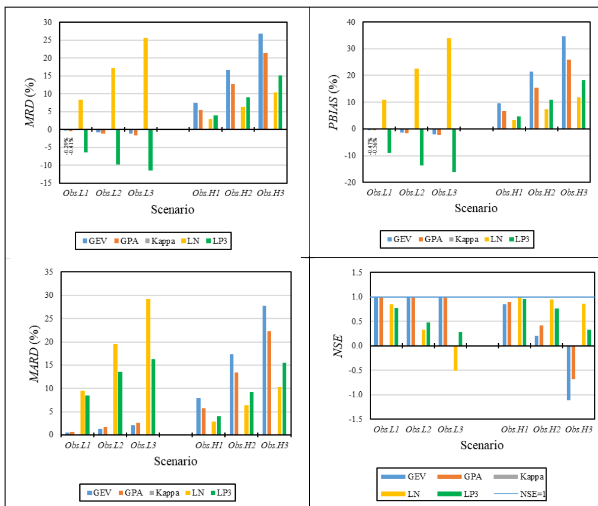
Figure B1.3 Impact of LO ( Obs.L1 , Obs.L2 and Obs.L3 ) and HO ( Obs.H1 , Obs.H2 and Obs.H3 ) scenarios on design rainfall estimated by different PDs from observed data for Rainfall Gauge 0025414
