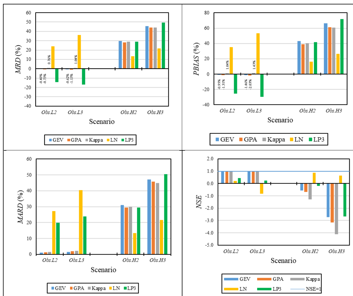
Figure B1.6 Impact of LO ( Obs.L2 and Obs.L3 ) and HO ( Obs.H2 and Obs.H3 ) scenarios on design floods estimated by different PDs from observed data in Catchment A2H012
