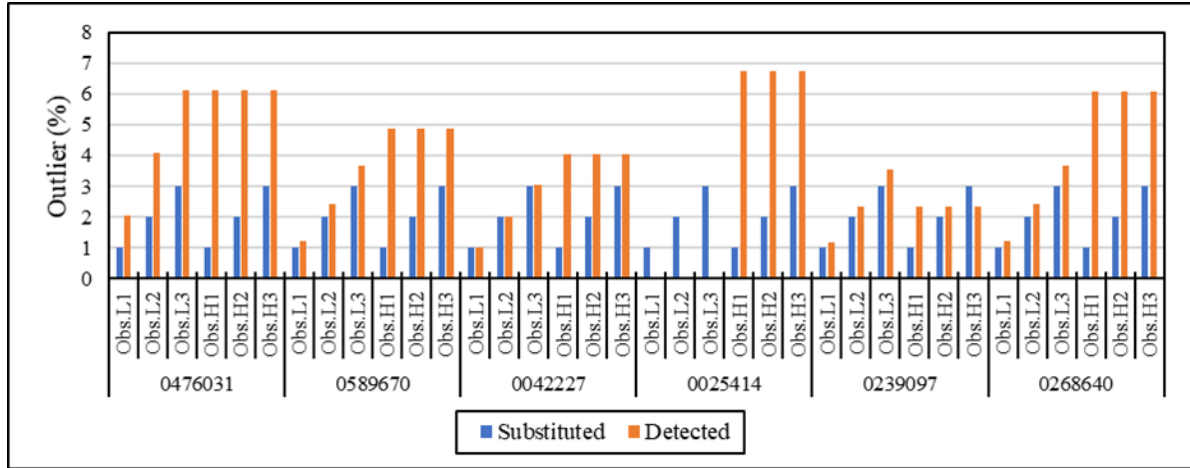
Figure 3.23 Percentage of substituted and detected outliers using the BP method on observed rainfall data with LO (Obs.L1, Obs.L2 and Obs.L3) and HO (Obs.H1, Obs.H2 and Obs.H3) scenarios
