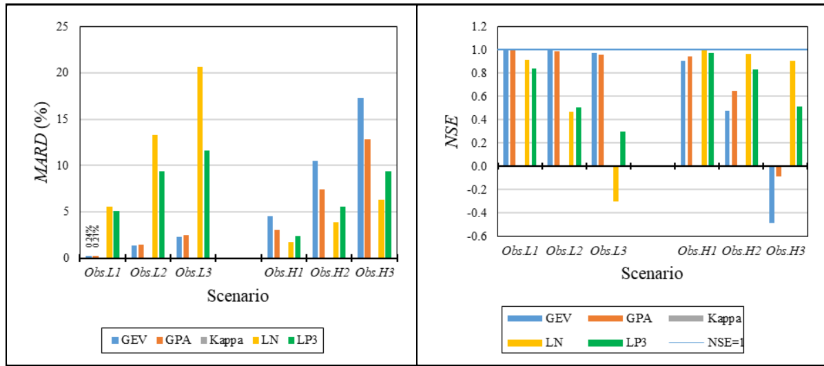
Figure 3.11 MARD and NSE for design rainfall events estimated using observed data for Rainfall Gauge 0042227 for LO (Obs.L1, Obs.L2 and Obs.L3) and HO (Obs.H1, Obs.H2 and Obs.H3) scenarios
