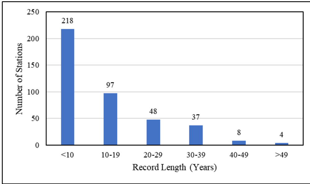
Figure 3.2 Distribution of record lengths in the short duration rainfall database for South Africa (after Smithers and Schulze, 2000a)
