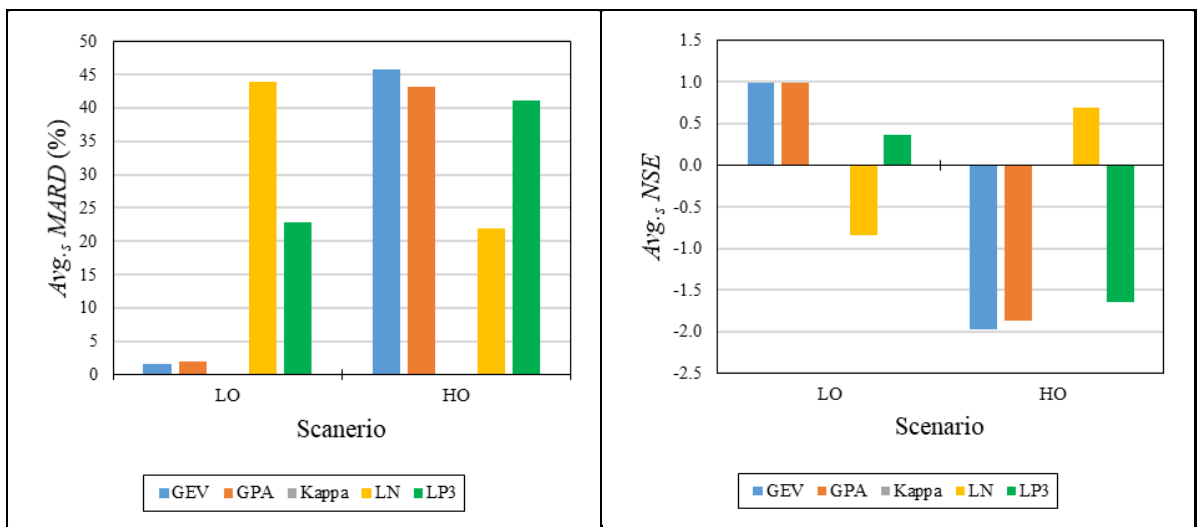
Figure 3.15 Avg.s MARD and Avg.s NSE for design flood events estimated using observed data with LOs and HOs
