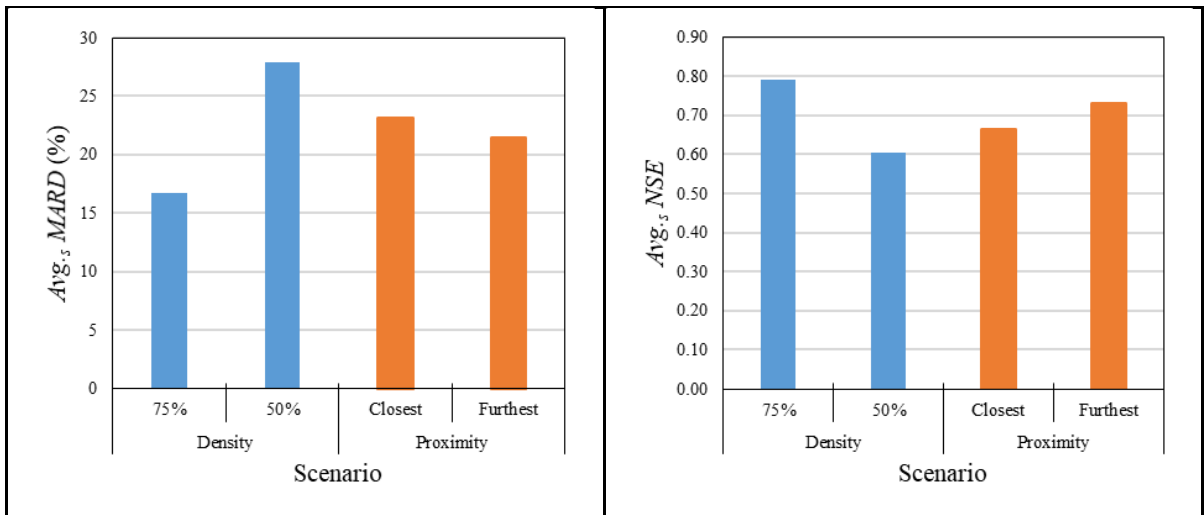
Figure 3.48 Avg.s MARD and Avg.s NSE for design flood events estimated using scenarios (Closest.75%, Closest.50%, Furthest.75% and Furthest.50%) of a systematically reduced gauge network
