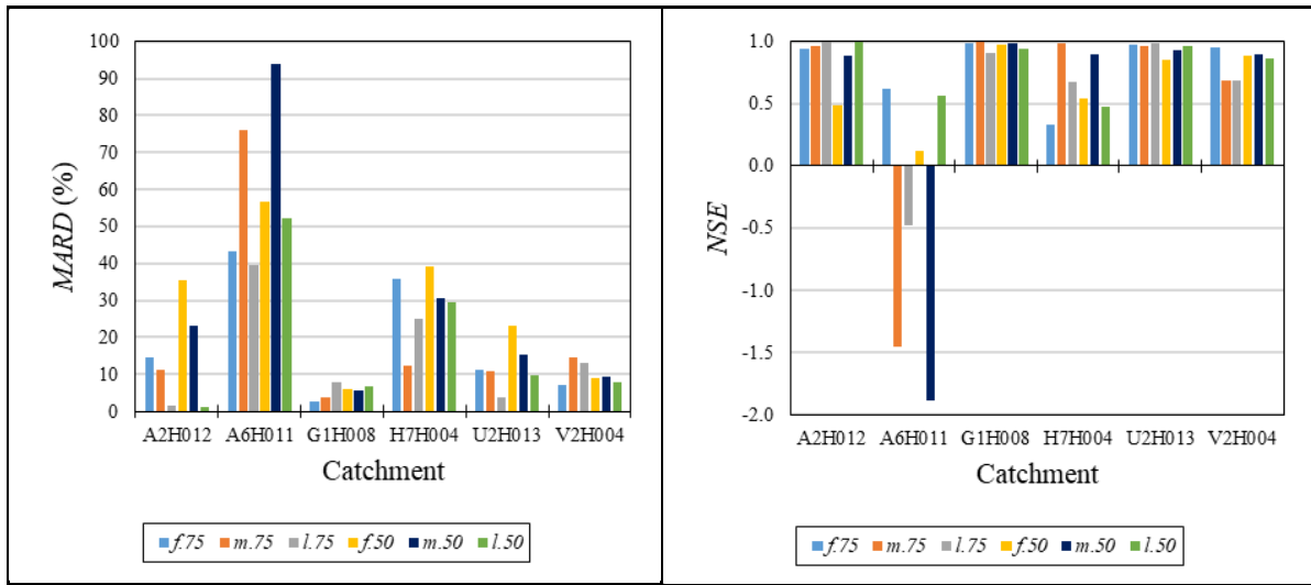
Figure 3.34 MARD and NSE for design flood events estimated using scenarios of 75% (f.75, m.75, l.75) and 50% (f.50, m.50, l.50) of record length
