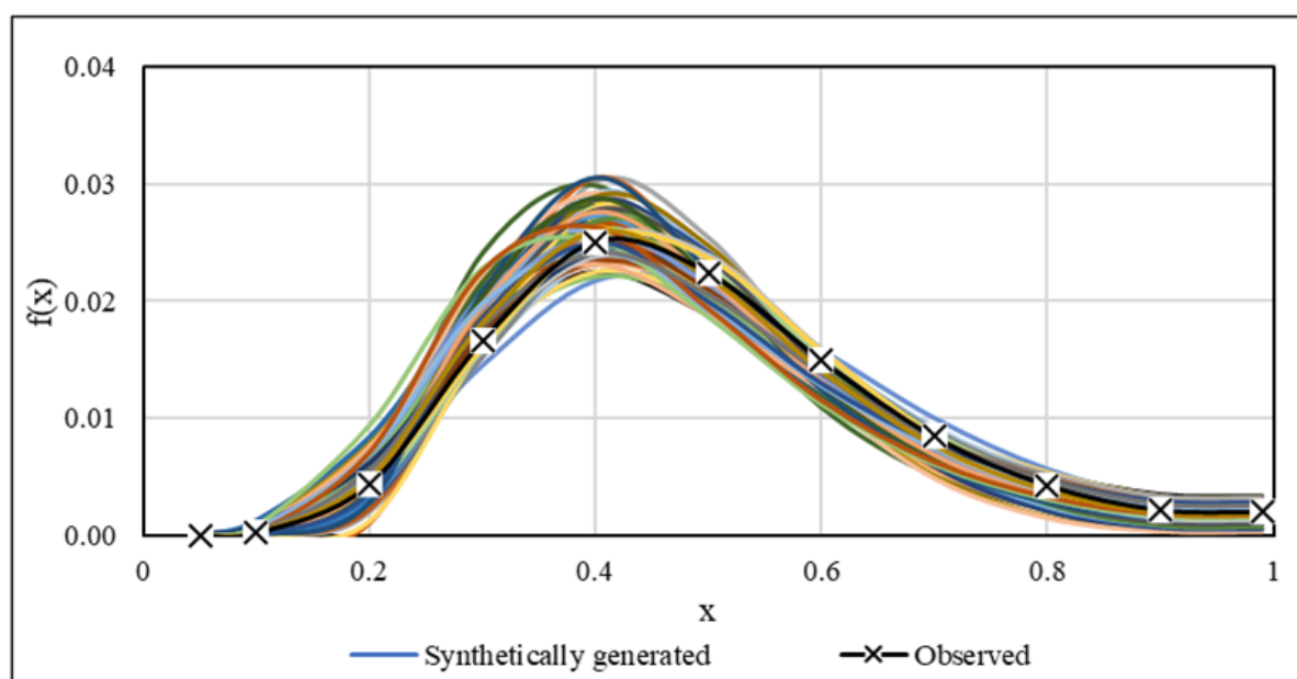
Figure 3.16 PDF for the observed and 100 synthetically generated rainfall data series at Rain Gauge 0268640
