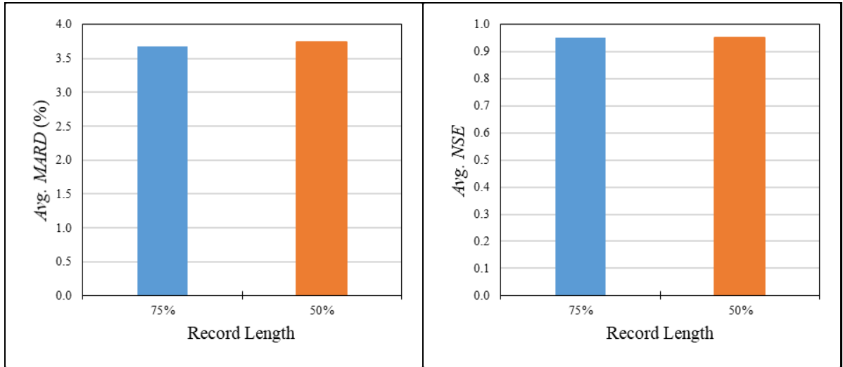
Figure 3.36 Avg. MARD and Avg. NSE for design rainfall events estimated using 75% and 50% of AMS records
