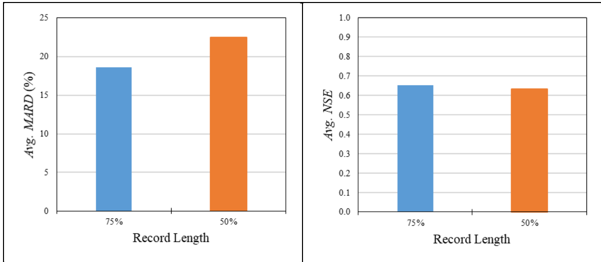
Figure 3.38 Avg. MARD and Avg. NSE for design flood events estimated using 75% and 50% of AMS records
