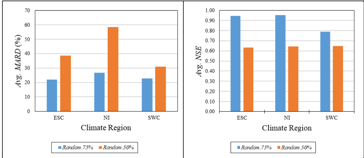
Figure 3.52 Avg. MRD and Avg. NSE of design flood events computed using a 75% and 50% randomly reduced gauge network
