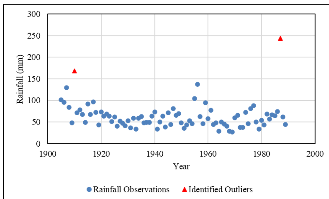
Figure 3.8 AMS plot for Driver Rainfall gauge 0239097 used in Catchment U2H013
