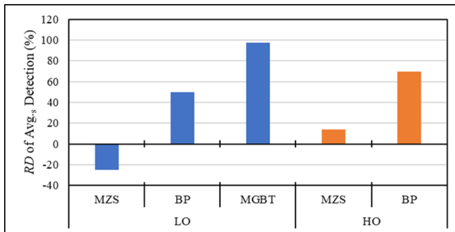
Figure 3.28 RD of Avg. Detection of LOs and HOs in synthetically generated rainfall data series using the BP, MZS and MGBT
