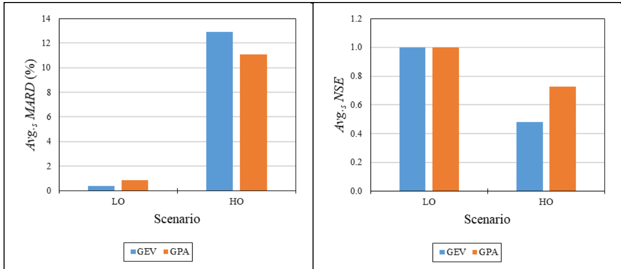
Figure 3.21 Avg.s\ MARD and Avg.s\ NSE for design flood events estimated using synthetically generated data with LOs and HOs
