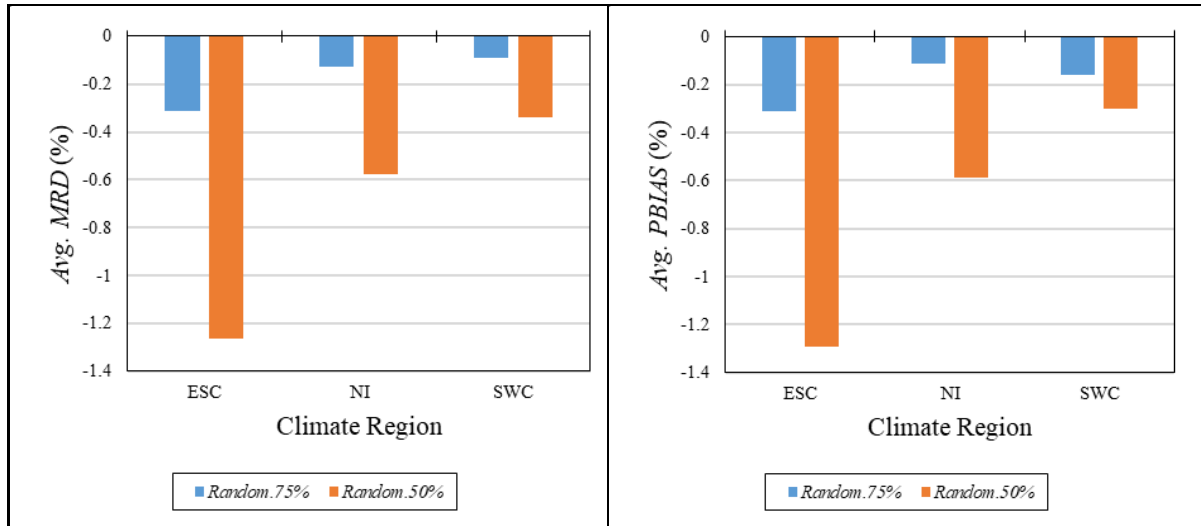
Figure 3.49 Avg. MRD and Avg. PBIAS of design rainfall events computed using a 75% and 50% randomly reduced gauge network
