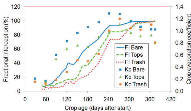
Figure 5 Measured fractional interception of photosynthetic active radiation as affected by different residue layers in the plant crop. Corresponding monthly average FAO crop evaporation coefficients ( Kc_{FAO} = ET_d/E_{crop} ) are presented by the symbols.
