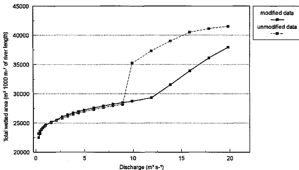
Figure 9.1 PHABSIM II predictions of change in total wetted area with discharge at Grootfontein, using data from transects GR695 and GR840. See text for details
