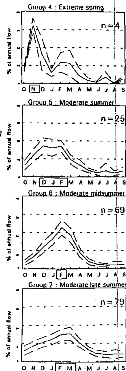
Figure 11.3 METHOD ONE: The distribution of the seven groups of gauging stations determined using an analysis of seasonal flow patterns. The dashed lines indicate plus and minus one standard deviation. The months of distinctive flow peaks are blocked
