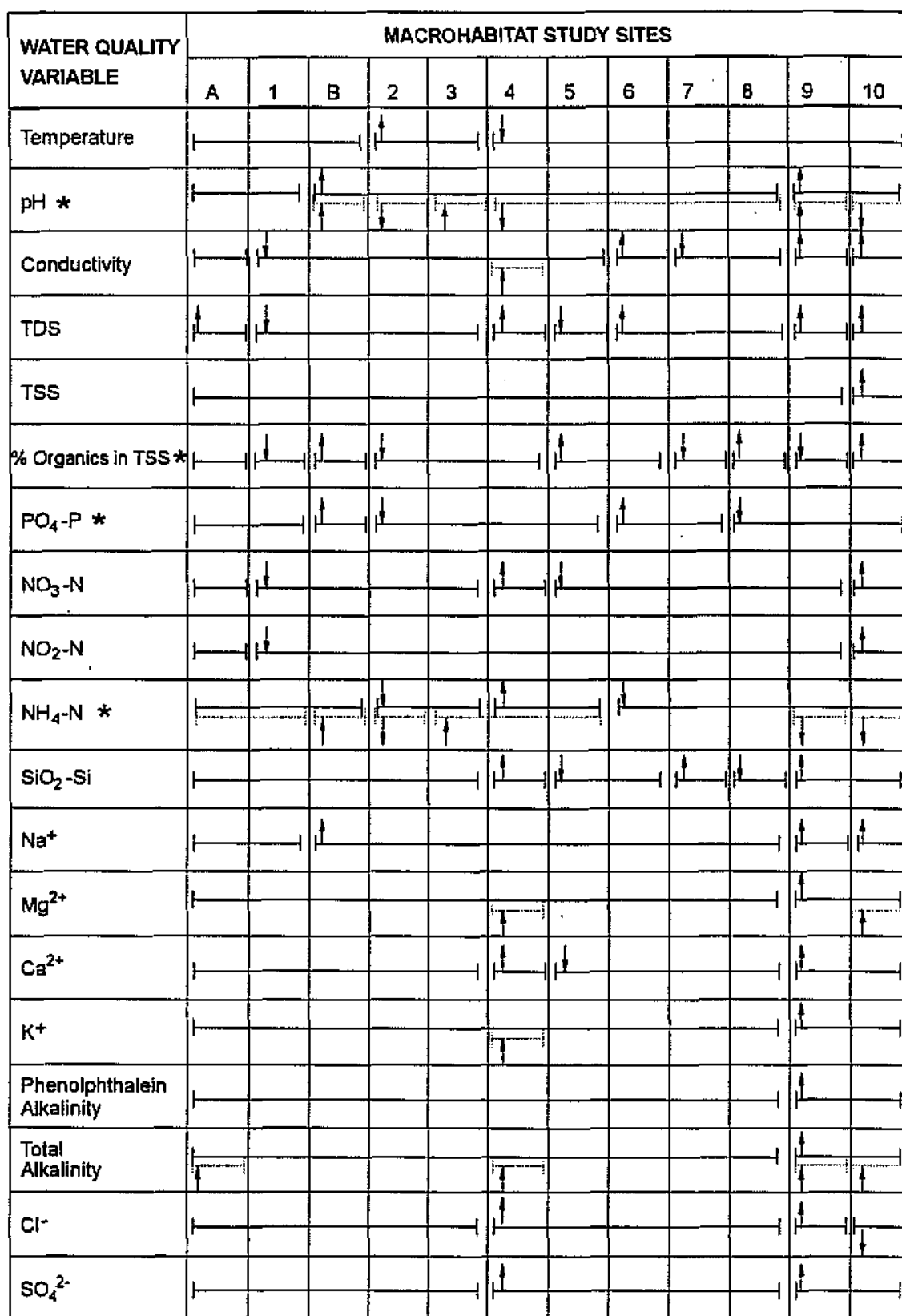
Figure 5.10 Large-scale trends (—) in water quality variables for the study area based on the summer data (February/March). ↑ indicates a noticeable increase in a water quality variable at a particular site, while ↓ indicates a decrease. These trends are not necessarily statistically significant. Asterisks represent those variables which exhibit highly variable longitudinal changes, and therefore, less obvious larger-scale trends. — represents a site(s) for which smaller-scale changes are apparent
