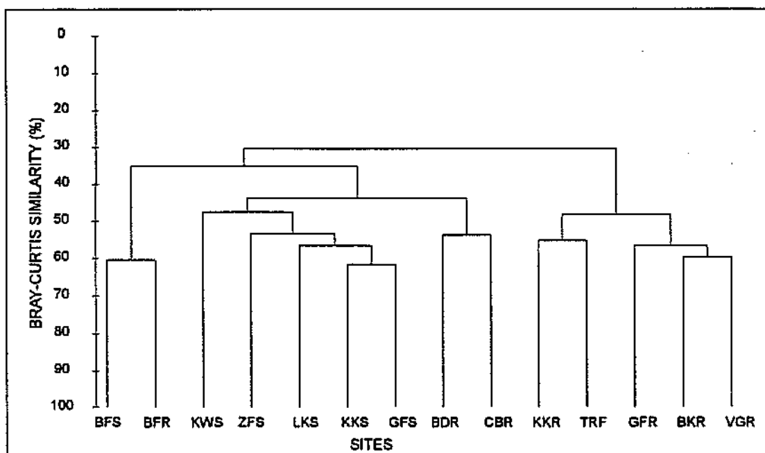
Figure 8.7 Dendrogram showing classification of the 11 macrohabitat sites of the study area based on mean sample abundances per species of benthic macroinvertebrates (summer data); samples from rock (R) and sand (S) bed areas were considered separately for sites with both types of substrate. Two main clusters of sites were distinguished at an arbitrary similarity level of 30% and six groups at 50%
