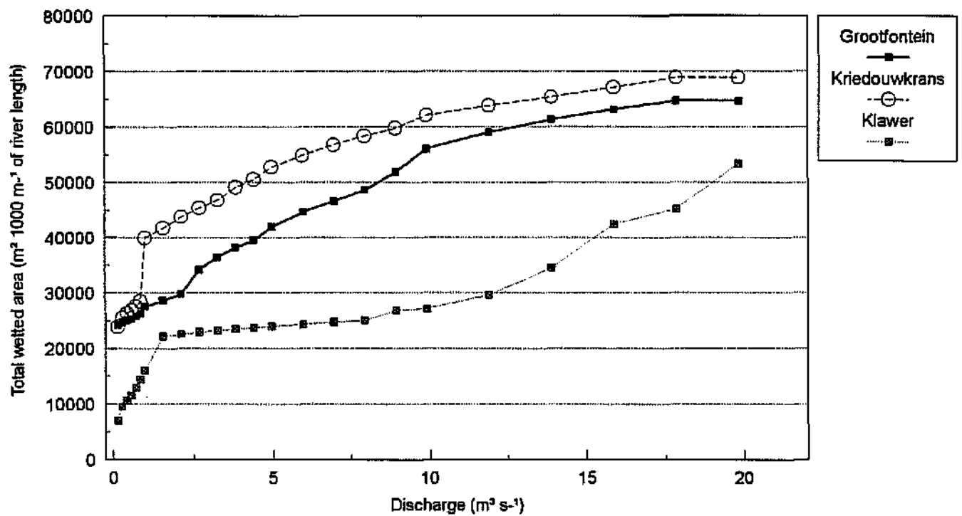
Figure 9.9 PHABSIM II predictions of change in total wetted area with discharge at Grootfontein, Kriedouwkrans and Klawer, using unmodified hydraulic data. See text for details
