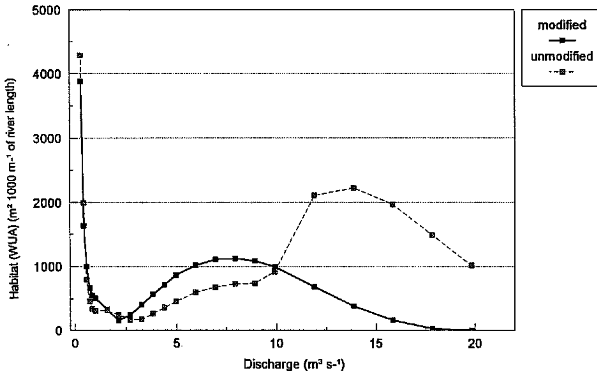
Figure 9.7 PHABSIM II predictions of change in WUA with discharge for the elmids larva Peloriolus granulosis (composite SI data) at Grootfontein, using data from transects GR695 and GR840. See text for details
