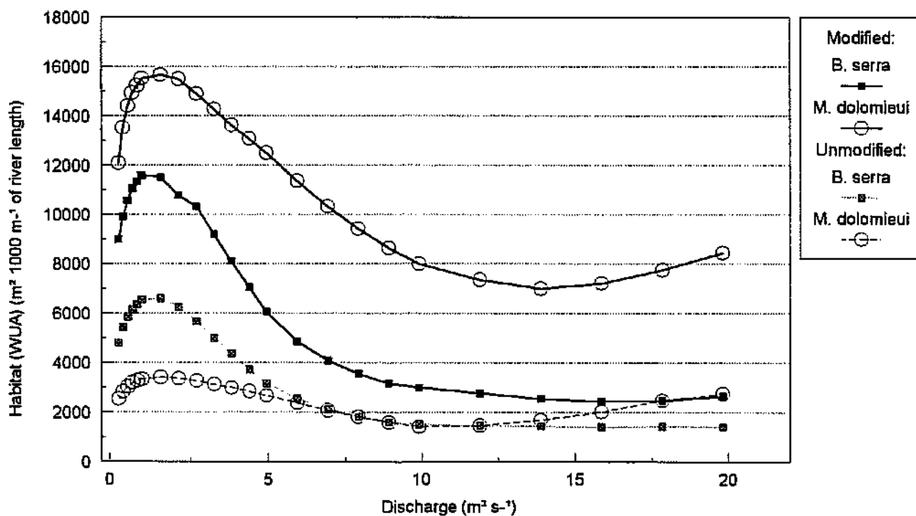
Figure 9.4 PHABSIM II predictions of change in WUA with discharge for Barbus serra and Micropterus dolomieu at Grootfontein, using data from transects GR695 and GR840. See text for details
