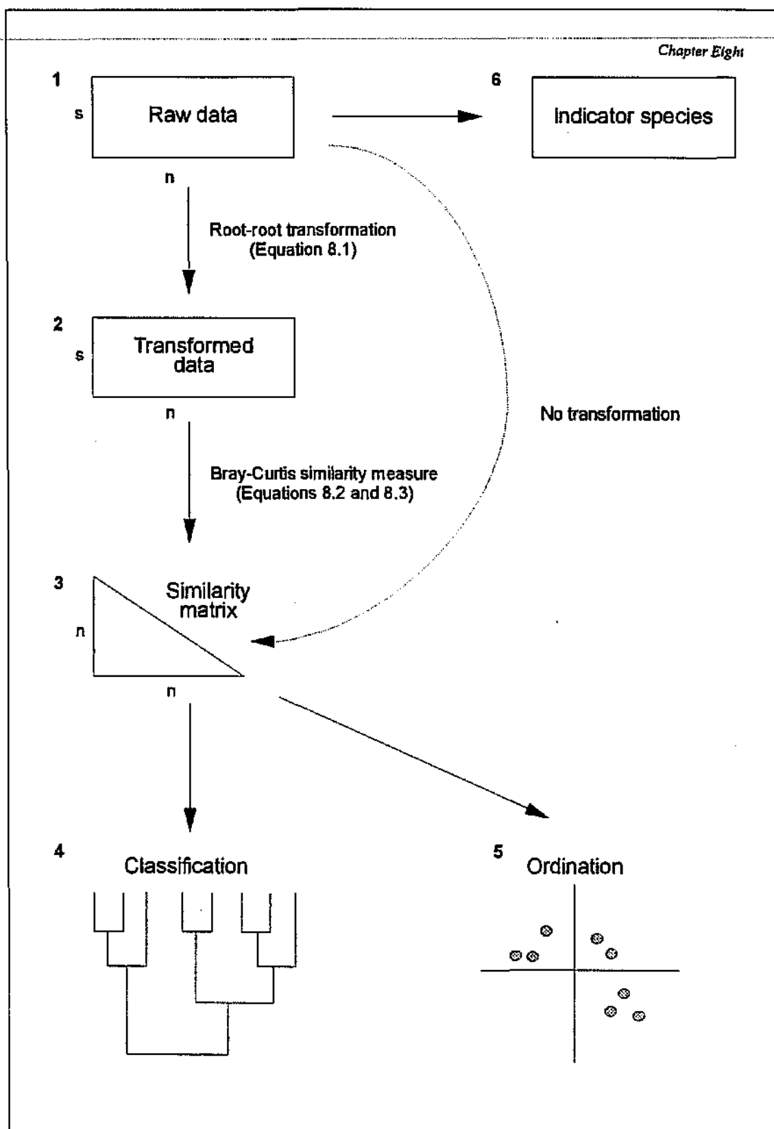
Figure 8.2 Diagrammatic summary of the stages of q-type analysis leading to classification and ordination of samples, and determination of indicator species (modified from Field et al. 1982). Raw data are represented in a matrix of n samples by s species (1). It may be necessary to transform the data (2). Comparison of each sample with every other sample using a measure of similarity produces a similarity matrix (3). Classification (4) and ordination (5) are complementary summaries of the relationships between eight samples in this diagram. Indicator species are obtained directly from the raw data (6)
