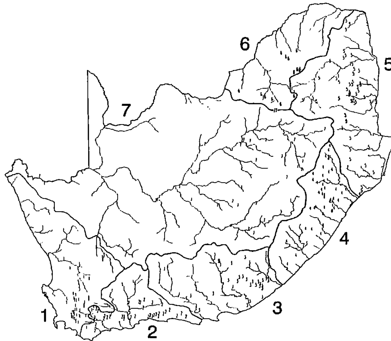
Figure 11.7 METHOD TWO: Map showing the locations of the stations used and the division of South Africa, Swaziland and Lesotho into seven regions based on correspondence analysis of monthly percentages of annual flow
