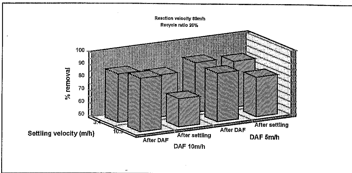
Figure 4: The influence of settling velocity and flotation velocity on suspended solids removal at a reaction zone velocity of 80 m/h and a recycle ratio of 20%.
