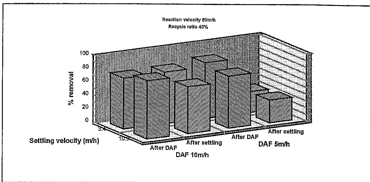
Figure 5: The influence of settling velocity and flotation velocity on suspended solids removal at a reaction zone velocity of 80 m/h and a recycle ratio of 40%.
