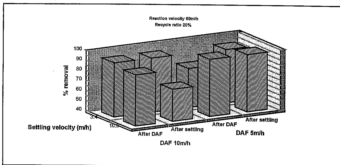
Figure 7: The influence of settling velocity and flotation velocity on ash content removal at a reaction zone velocity of 80 m/h and a recycle ratio of 20%.
