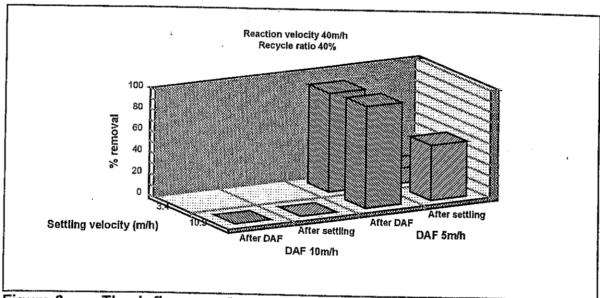
Figure 6: The influence of settling velocity and flotation velocity on ash content removal at a reaction zone velocity of 40 m/h and a recycle ratio of 40%.
