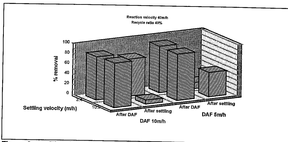
Figure 3: The influence of settling velocity and flotation velocity on suspended solids removal at a reaction zone velocity of 40 m/h and a recycle ratio of 40%.
