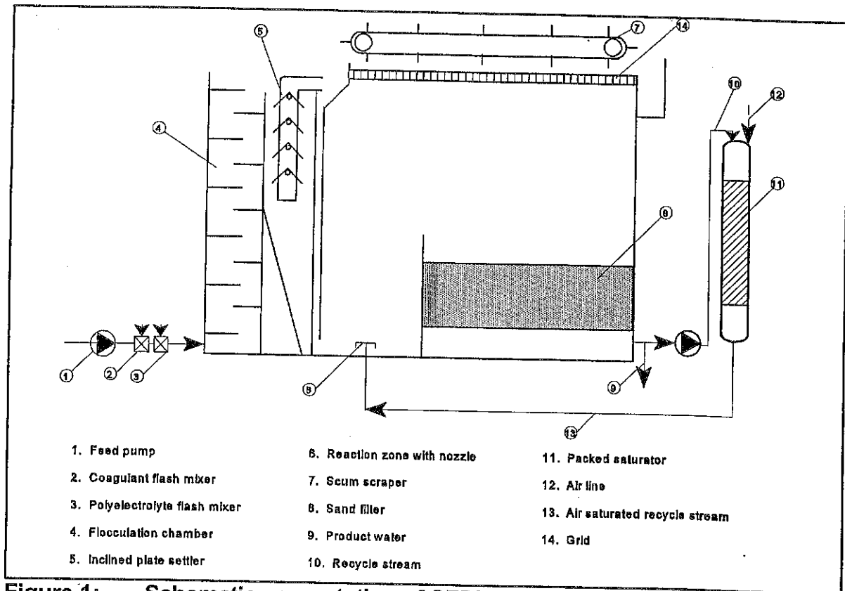
Figure 1: Schematic presentation of SEDIDAF pilot plant
