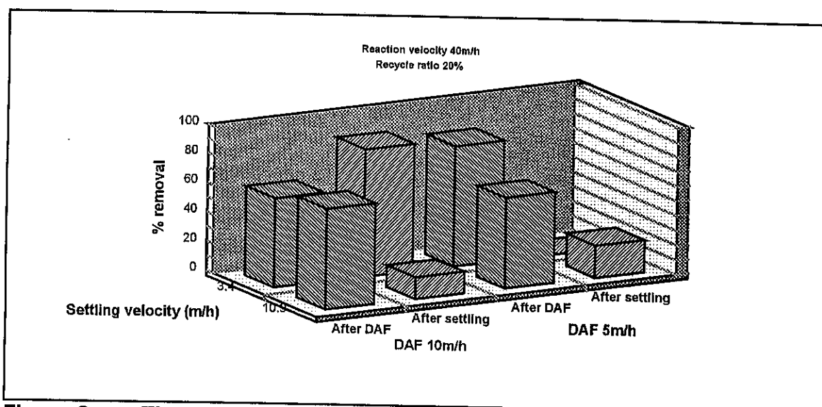
Figure 2: The influence of settling velocity and flotation velocity on suspended solids removal at a reaction zone velocity of 40 m/h and a recycle ratio of 20%.
