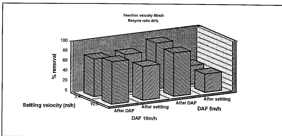
Figure 8: The influence of settling velocity and flotation velocity on ash content removal at a reaction zone velocity of 80 m/h and a recycle ratio of 40%.
