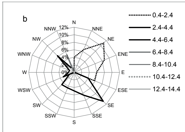
Figure 3 Wind speed (m \cdot s ^{-1} ) and wind direction at (a) Somerton farm and (b) Truro farm during the field campaign
