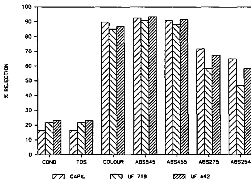
FIGURE 3.20 : COMPARISON OF PERMEATE QUALITIES - COLOUR REMOVAL FROM WATER
