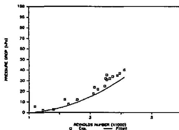
FIGURE 3.4 : EXPERIMENTAL AND FITTED PRESSURE DROP DATA AT VARIOUS Re -NUMBERS - MODULE N150L300
