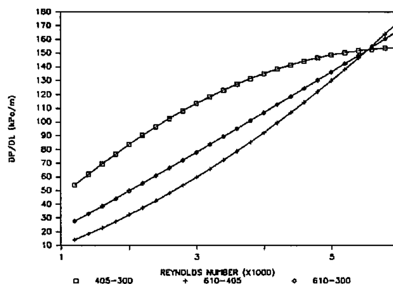
FIGURE 3.8 : PLOT OF CALCULATED LENGTH COMPONENT OF PRESSURE DROP - \Delta P/\Delta L150
