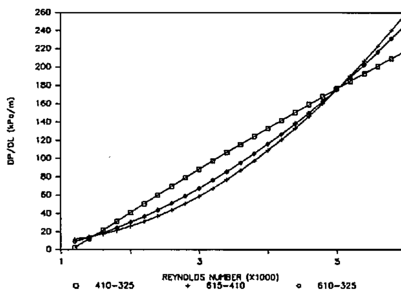
FIGURE 3.7 : PLOT OF CALCULATED LENGTH COMPONENT OF PRESSURE DROP - \Delta P/\Delta L100
