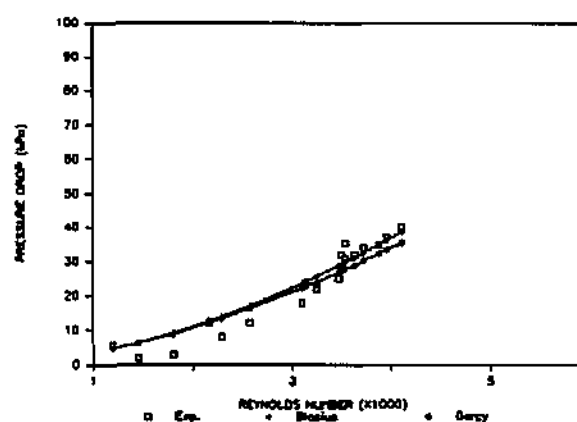
FIGURE 3.15 : COMPARISON OF EXPERIMENTAL AND SIMULATED PRESSURE DROP - MODULE N150L300
