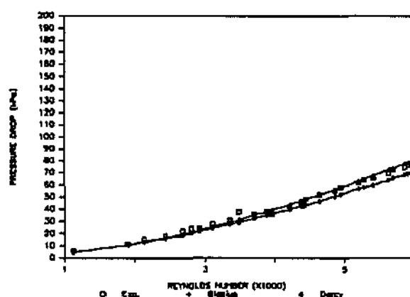
FIGURE 3.12 : COMPARISON OF EXPERIMENTAL AND SIMULATED PRESSURE DROP - MODULE N100L325
