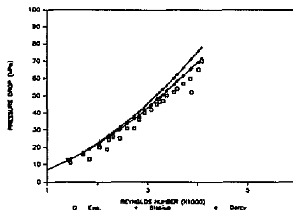
FIGURE 3.17 : COMPARISON OF EXPERIMENTAL AND SIMULATED PRESSURE DROP - MODULE N150L610
