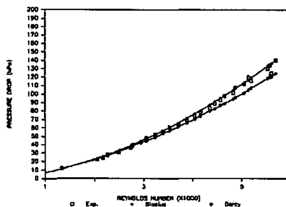
FIGURE 3.14 : COMPARISON OF EXPERIMENTAL AND SIMULATED PRESSURE DROP - MODULE N100L615
