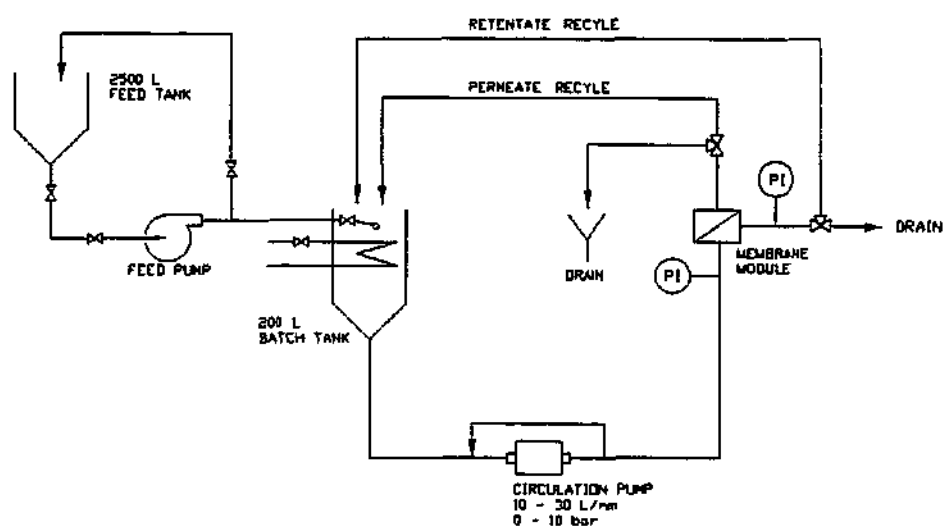
FIGURE 2.3 : SCHEMATIC OF EXPERIMENTAL EQUIPMENT USED IN COLOUR REMOVAL FROM WATER
