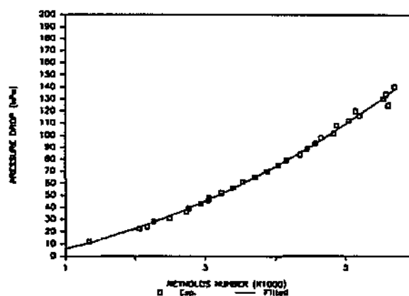
FIGURE 3.3 : EXPERIMENTAL AND FITTED PRESSURE DROP DATA AT VARIOUS Re -NUMBERS - MODULE N100L615
