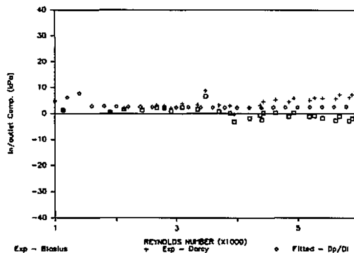
FIGURE 3.10 : \Delta P_{ends} COMPONENT FOR N100L325 MODULE
