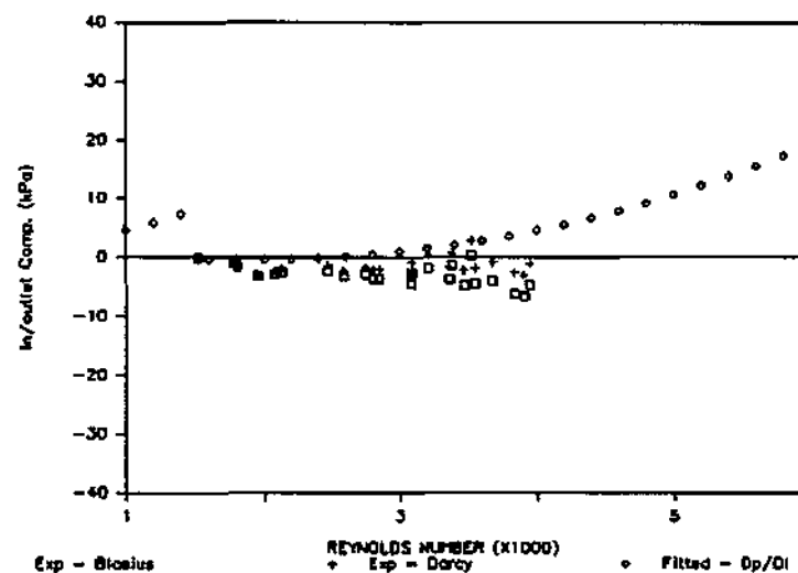
FIGURE 3.11 : \Delta P_{ends} COMPONENT FOR N150L405 MODULE
