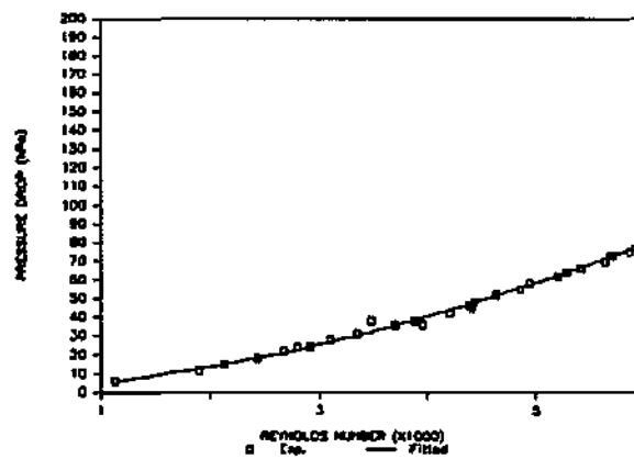
FIGURE 3.1 : EXPERIMENTAL AND FITTED PRESSURE DROP DATA AT VARIOUS Re -NUMBERS - MODULE N100L325
