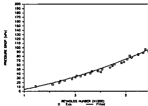
FIGURE 3.2 : EXPERIMENTAL AND FITTED PRESSURE DROP DATA AT VARIOUS Re -NUMBERS - MODULE N100L410
