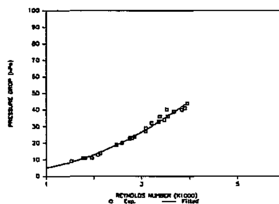
FIGURE 3.5 : EXPERIMENTAL AND FITTED PRESSURE DROP DATA AT VARIOUS Re -NUMBERS - MODULE N150L405
