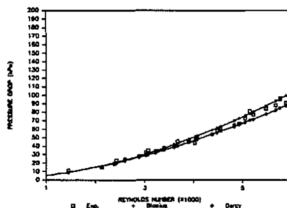
FIGURE 3.13 : COMPARISON OF EXPERIMENTAL AND SIMULATED PRESSURE DROP - MODULE N100L410
