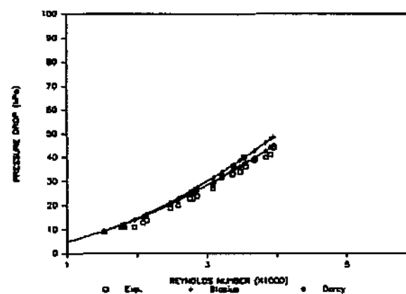
FIGURE 3.16 : COMPARISON OF EXPERIMENTAL AND SIMULATED PRESSURE DROP - MODULE N150L405
