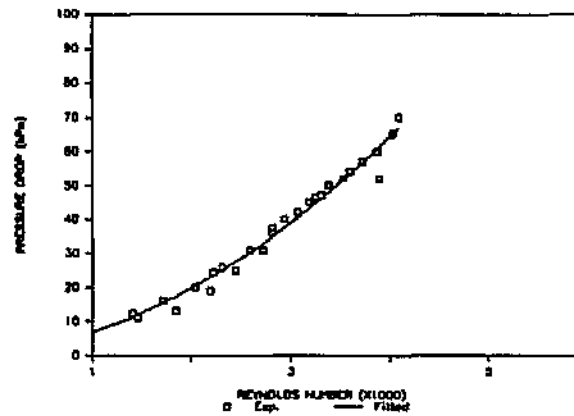
FIGURE 3.6 : EXPERIMENTAL AND FITTED PRESSURE DROP DATA AT VARIOUS Re -NUMBERS - MODULE N150L610
