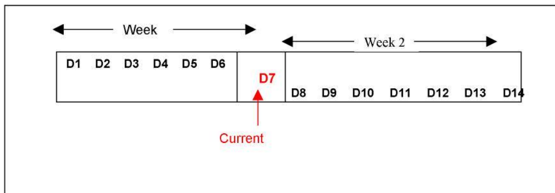
Figure 9.3: DISA Scheduling
