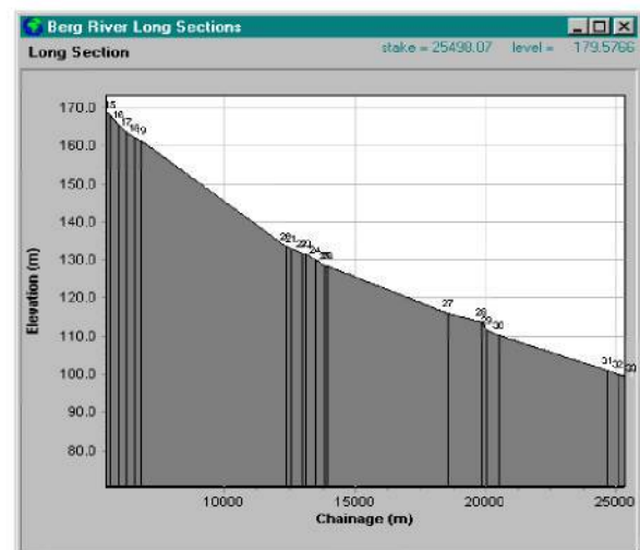
Figure 7.4: Long Section
