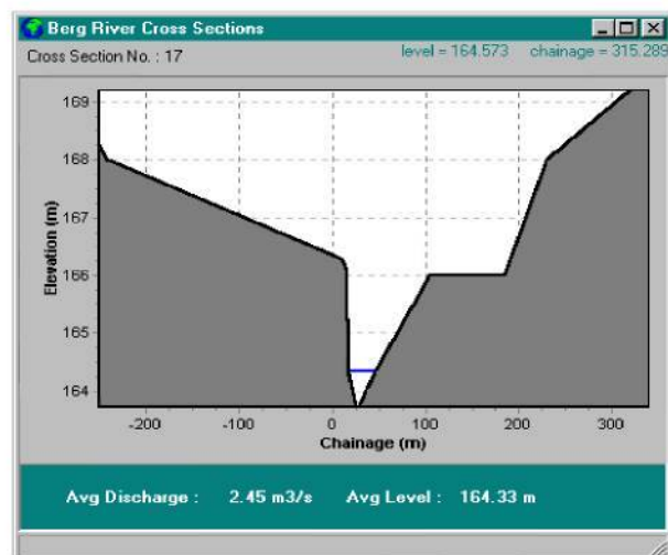
Figure 7.3: Cross Section
