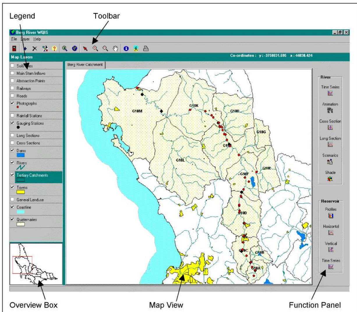
Figure 7.7: Main Screen
