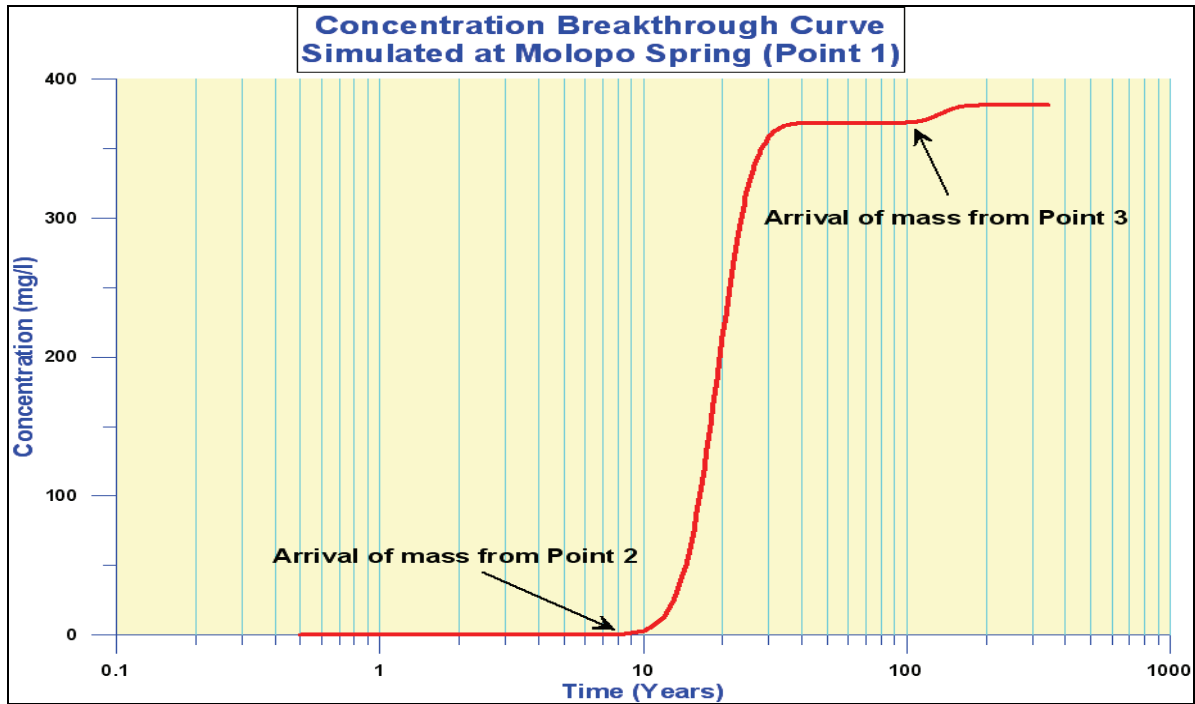
Figure 26 – The response of tracer injections at point 2 and 3 in the 3D simulation model, to derive the travel time of pollution in the aquifer. The points 2 and 3 are respectively 8 and 18.5 km from the spring outlet.
