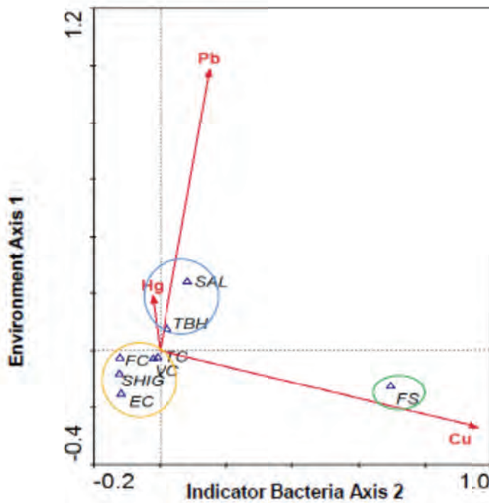
Figure 3.6 CCA ordination plot for the heavy metal quality variables and the total bacterial growth at the five study sites and during autumn, winter, spring and summer seasons. Abbreviations: Sites 1 = Umgeni River mouth, 2 = Informal settlement at Reservoir Hills, 3 = New Germany Waste Treatment Works, 4 = Krantzklouf Nature Reserve, 5 = Inanda Dam. Seasons: A = Autumn, W = Winter, Sp = Spring, S = Summer.
