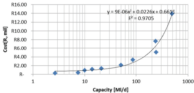
Figure 6.23: Operating cost curve for chemical costs – all capacities
