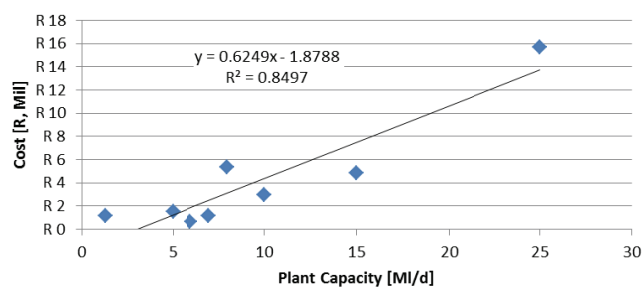
Figure 6.19: Capital cost curve for P&G – up to 25 ML/d
