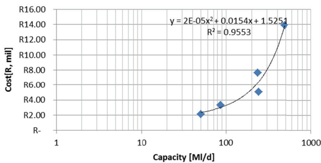
Figure 6.25: Operating cost curve for chemical costs – 50 ML/d to 500 ML/d
