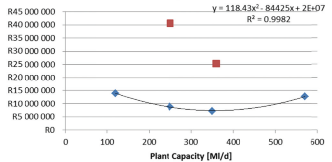
Figure 6.22: Operating cost curve for HR – 120 ML/d to 570 ML/d
