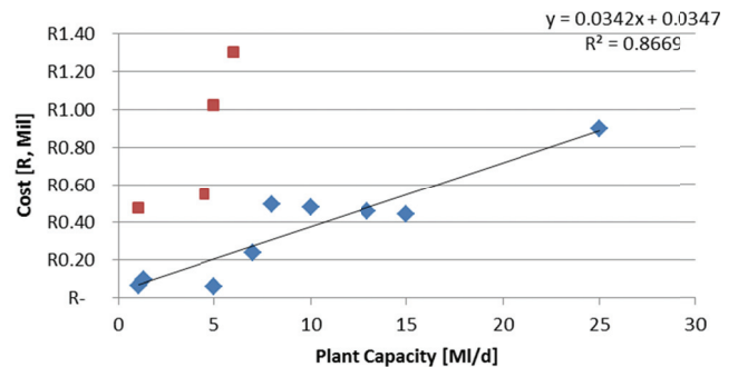
Figure 6.15: Capital cost curve for chlorination – 1 ML/d to 25 ML/d
