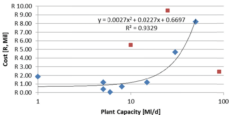
Figure 6.1: Capital cost curve for inlet distribution works of less than 50 ML/d
