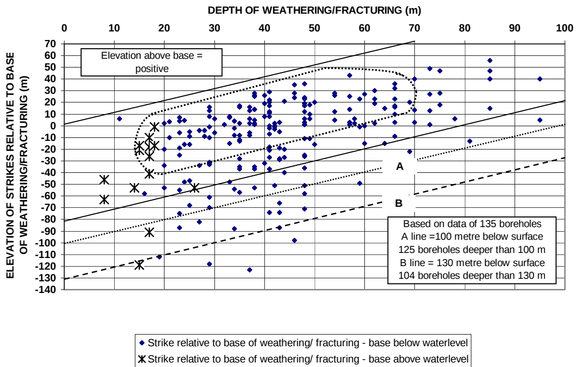
FIGURE 19 RELATION BETWEEN WATER STRIKES AND BASE OF WEATHERING AND FRACTURING BATHOLITH PROJECT
