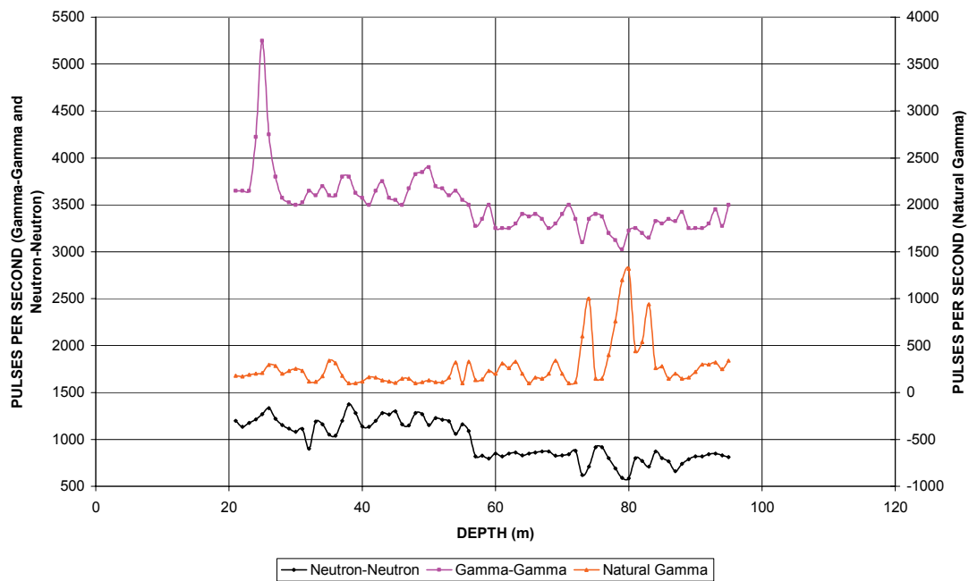
FIGURE 28 GAMMA-GAMMA, NATURAL GAMMA AND NEUTRON-NEUTRON LOGS OF BOREHOLE MON 12 VAALPUTS
