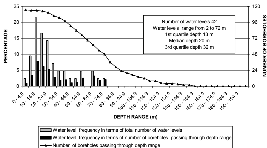
FIGURE 20b DISTRIBUTION OF WATER LEVELS SUBDIVISION 12
