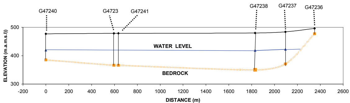
FIGURE 10 SECTION THROUGH CAINOZOIC DEPOSITS ALONG STEINKOPF - GOODHOUSE ROAD 13 KM UPSTREAM OF HENKRIES SPRING
