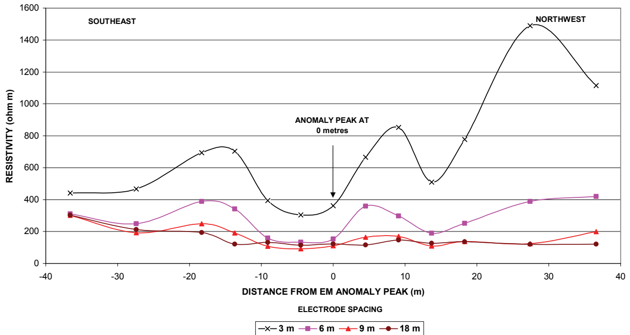
FIGURE 38f HORIZONTAL WENNER PROFILING ACROSS EM ANOMALY DROOGE GROND 135 DISTRICT KENHARDT
