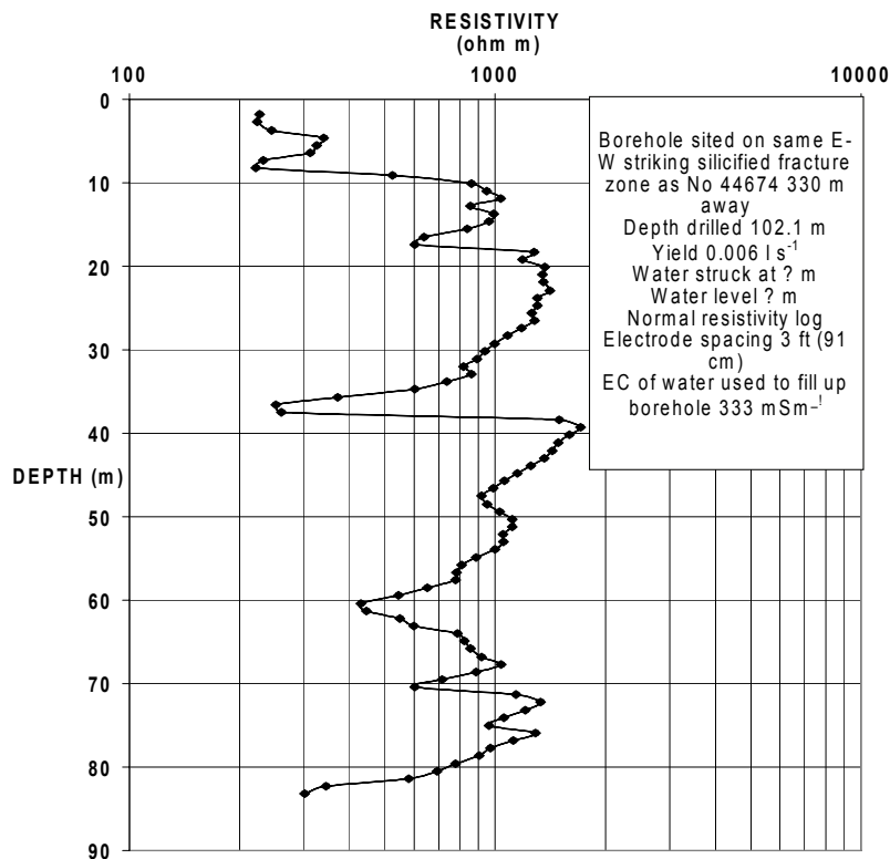
FIGURE 35a ELECTRICAL RESISTIVITY LOG OF BOREHOLE No 36508 (G2512) HELDUM PORTION OF LUCAS VLEI 93
