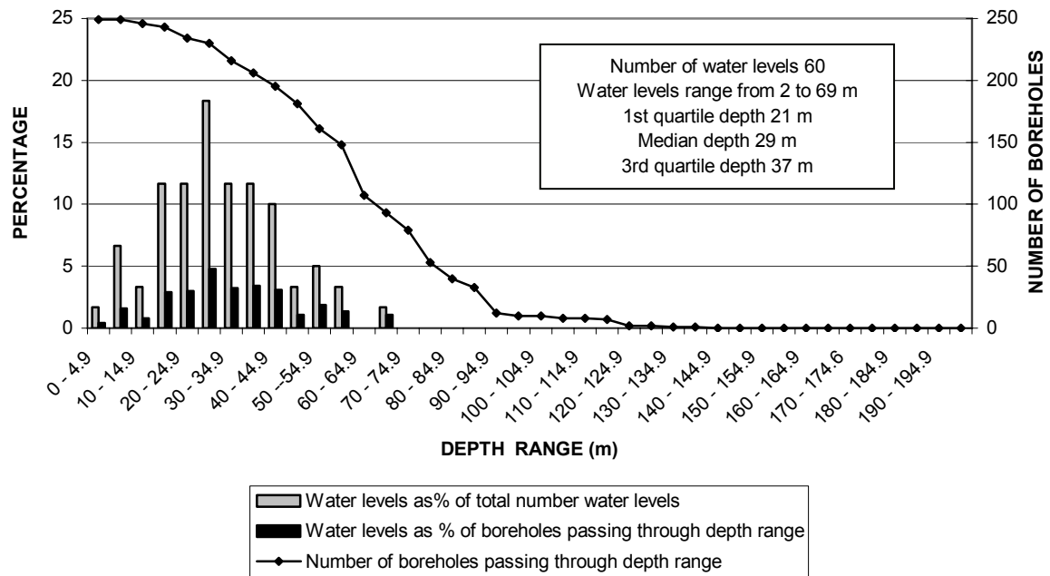
FIGURE16b DISTRIBUTION OF WATER LEVELS SUBDIVISION 8
