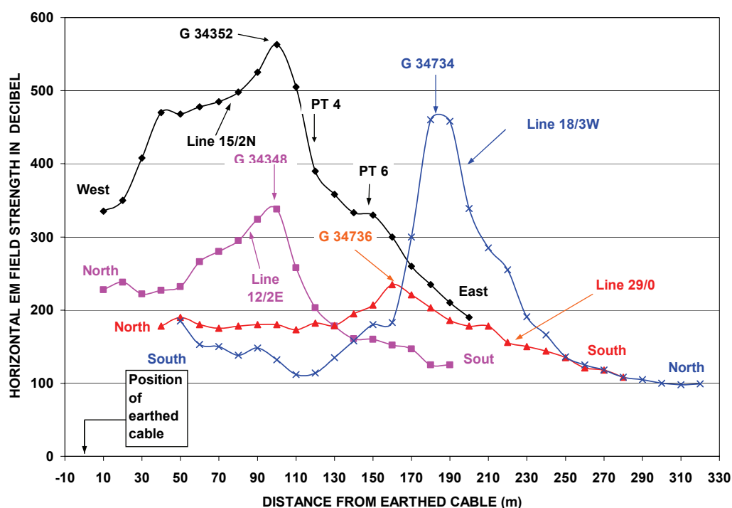
FIGURE 41b ELECTROMAGNETIC ANOMALIES ACROSS LINEAMENTS POFADDER TOWN LANDS
