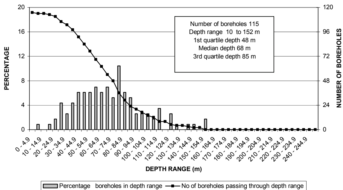
FIGURE 20a DISTRIBUTION OF BOREHOLE DEPTHS SUBDIVISION 12
