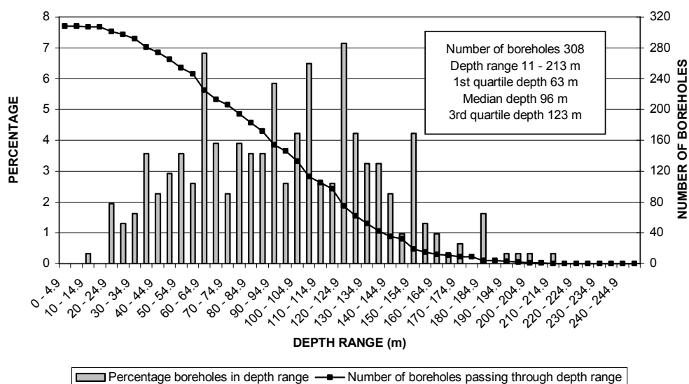
FIGURE 19a DISTRIBUTION OF BOREHOLE DEPTHS SUBDIVISION 11
