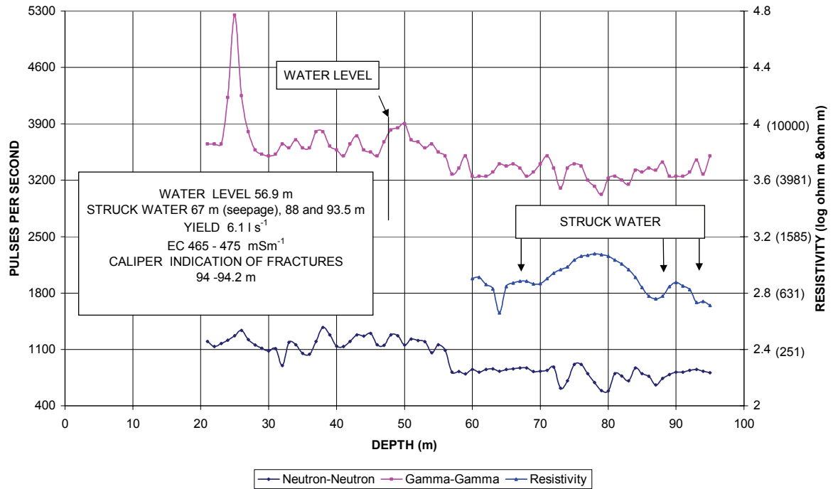
FIGURE 27 GAMMA-GAMMA, ELECTRICAL RESISTIVITY AND NEUTRON-NEUTRON LOGS OF BOREHOLE MON 12 VAALPUTS
