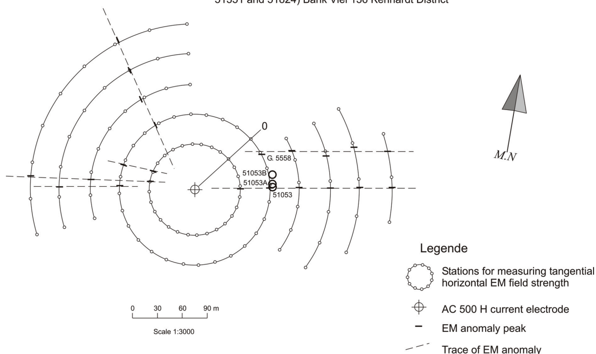
Figure 39a: Electromagnetic survey at borehole site G 5558 (Borehole No's 51053, 51351 and 51824) Bank Vlei 136 Kenhardt District
