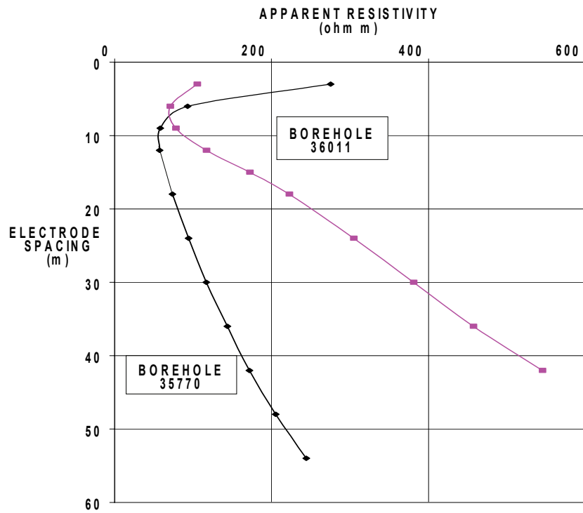
FIGURE 34b WENNER DEPTH PROBES AT BOREHOLES No's 35770 (G 503) AND 36011 (G 2644)
