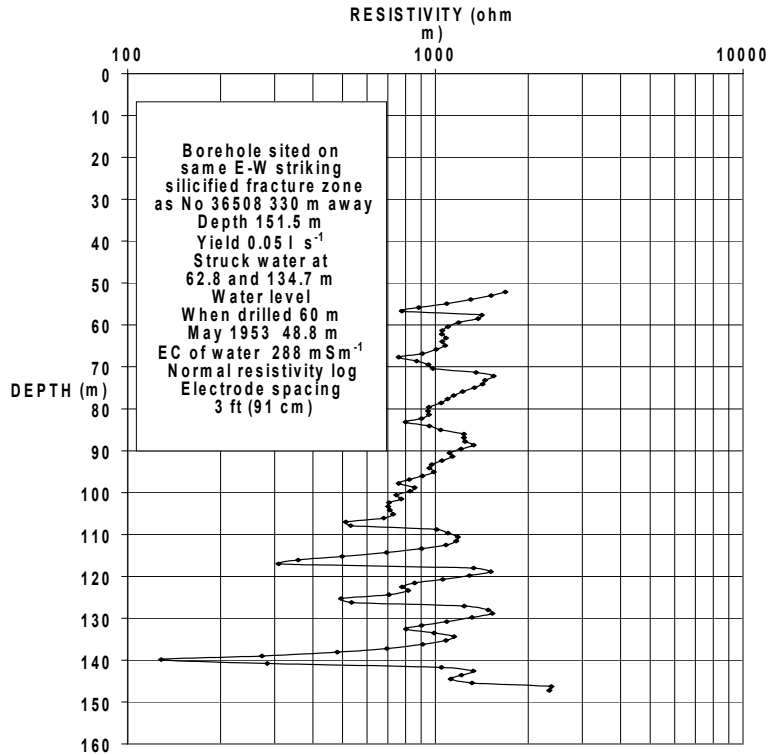
FIGURE 35b ELECTRICAL RESISTIVITY LOG OF BOREHOLE No 44674 HELLUM PT. LUCAS VLEI 93
