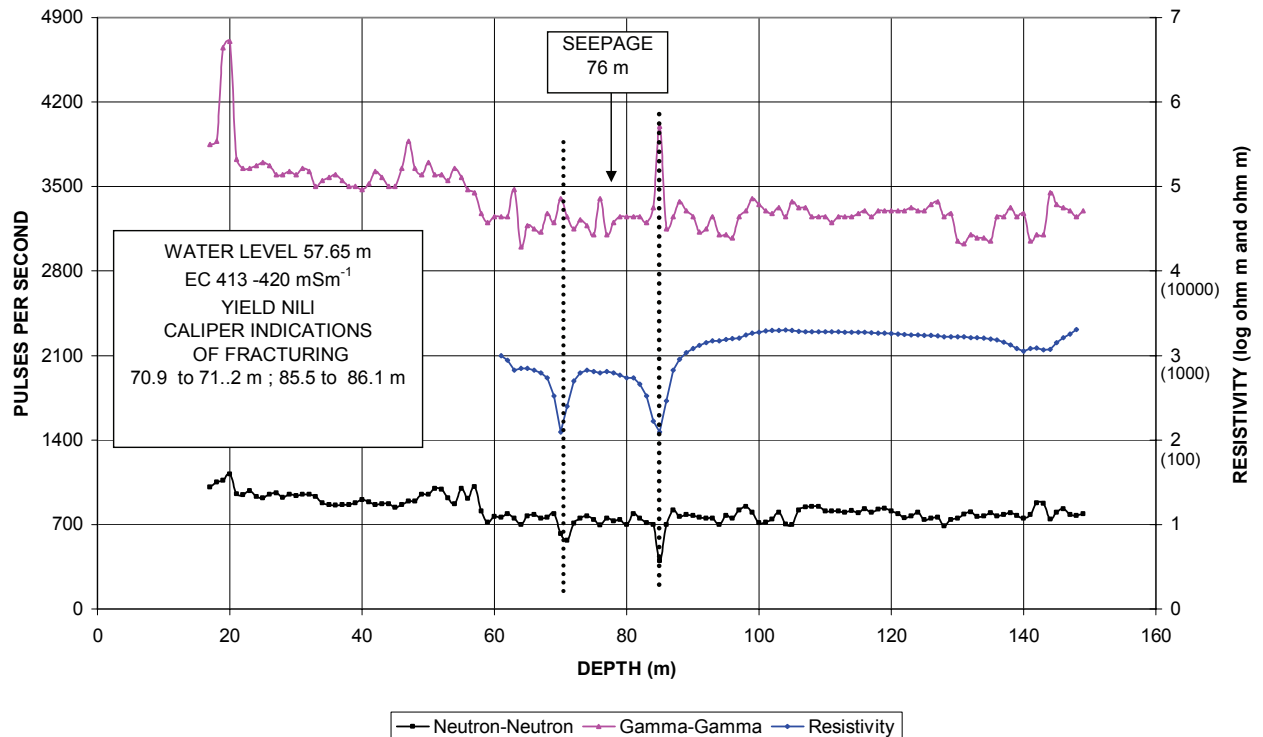
FIGURE 30 GAMMA-GAMMA, ELECTRICAL RESISTIVITY AND NEUTRON-NEUTRON LOGS BOREHOLE MON 15 VAALPUTS
