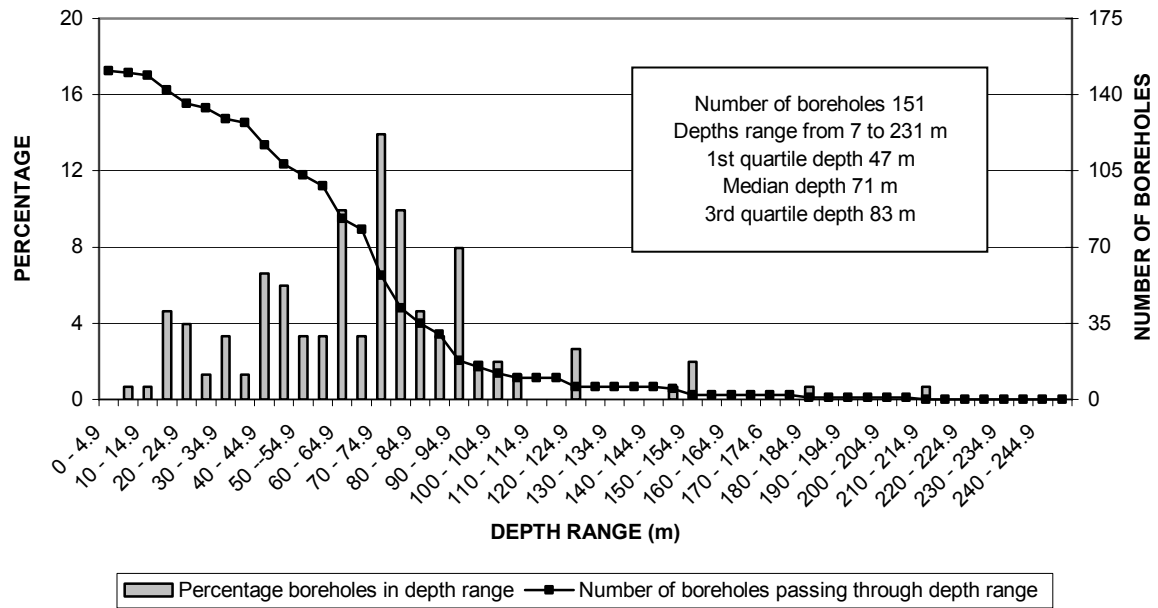
FIGURE 15a DISTRIBUTION OF BOREHOLE DEPTHS SUBDIVISION 7
