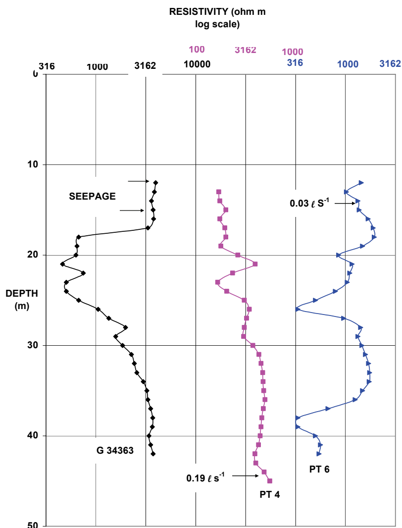
FIGURE 41e E. R. LOGS OF BOREHOLES G 34353 . PT 4 AND PT 6 LOCLITY B, POFADDER
