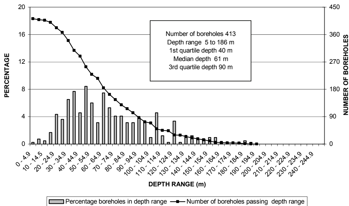
FIGURE14a DISTRIBUTION OF BOREHOLE DEPTHS SUBDIVISION 6
