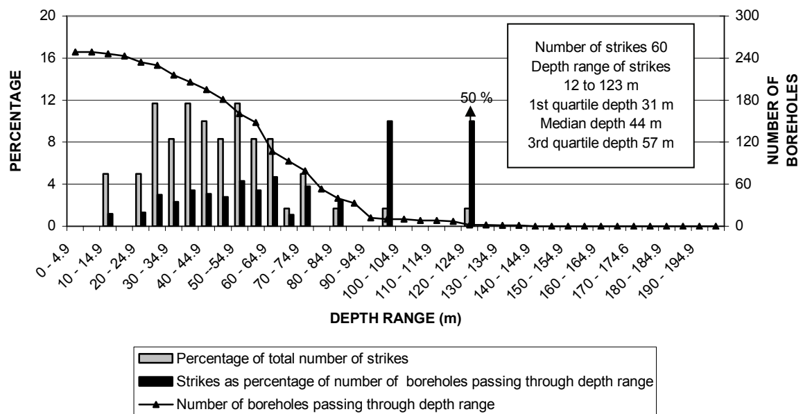
FIGURE16c DISTRIBUTION OF STRIKES BELOW SURFACE SUBDIVISION 8
