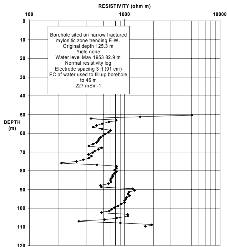
FIGURE 36c ELECTRICAL RESISTIVITY LOG OF BOREHOLE No 37093 (G2648) HELSUM PORTION OF LUCAS Vlei 93
