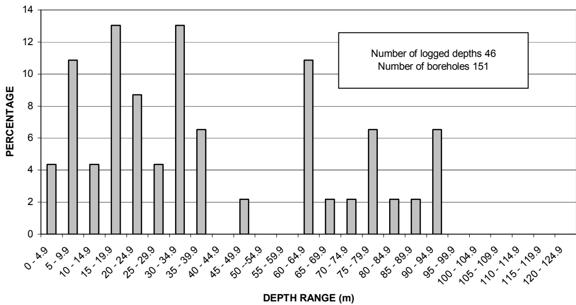
FIGURE 15d DISTRIBUTION OF LOGGED DEPTHS OF WEATHERING AND FRACTURING SUBDIVISION 7
