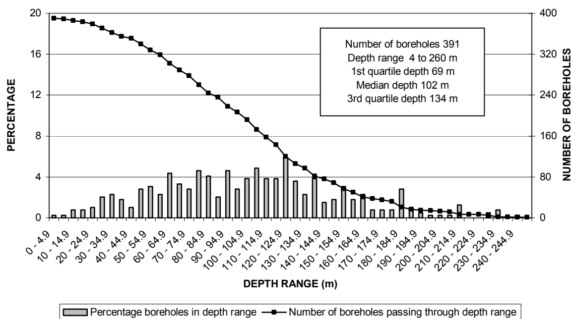
FIGURE 21a DISTRIBUTION OF BOREHOLE DEPTHS SUBDIVISION 14
