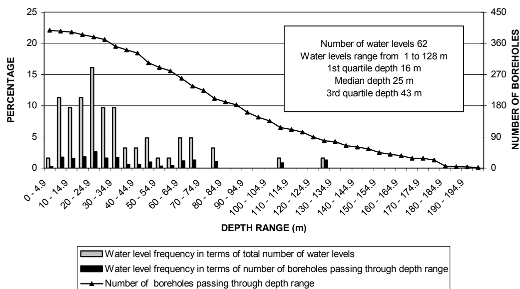
FIGURE18b DISTRIBUTION OF WATER LEVELS SUBDIVISION 10
