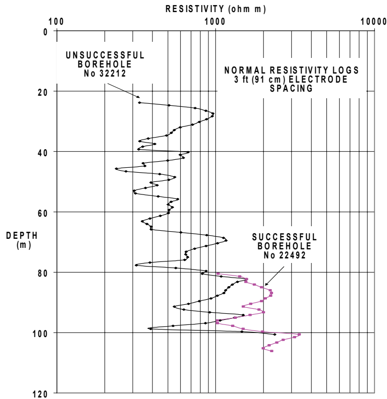
FIGURE 42 E. R. LOGS OF TWO BOREHOLES LONGZIEK VLEI 151 DISTRICT KENHARDT
