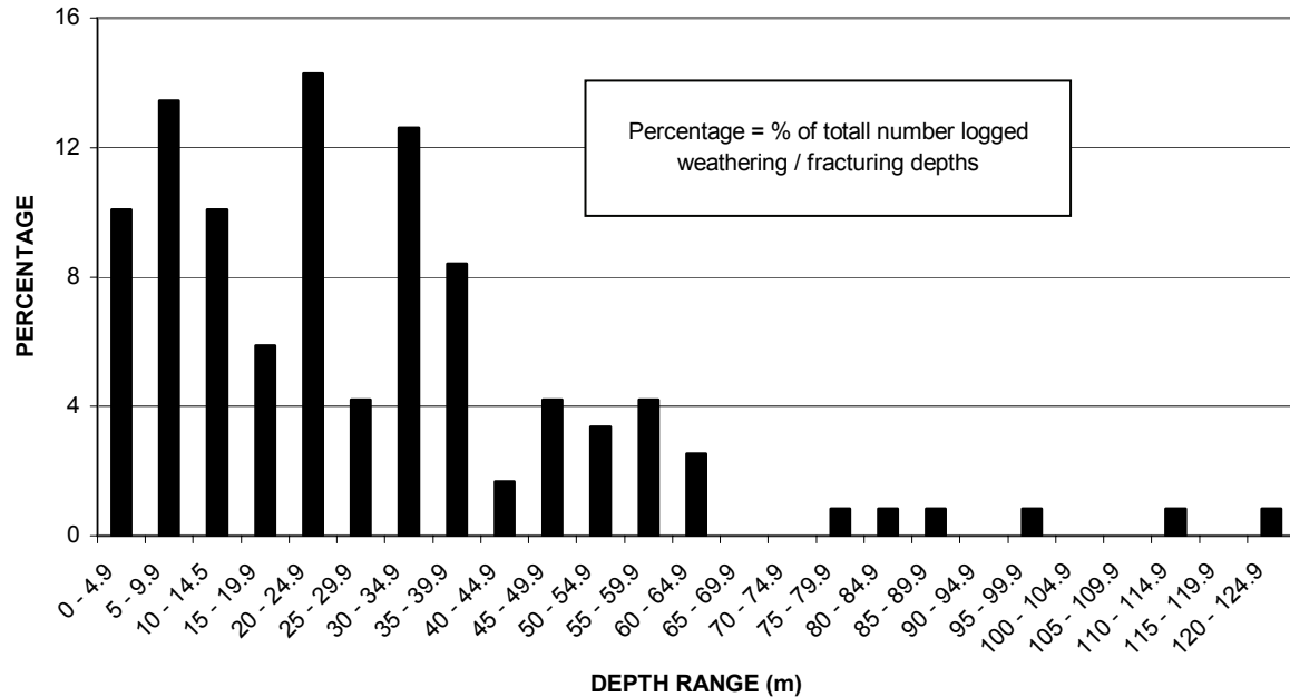
FIGURE 14d DISTRIBUTION OF LOGGED WEATHERING /FRACTURING DEPTHS SUBDIVISION 6
