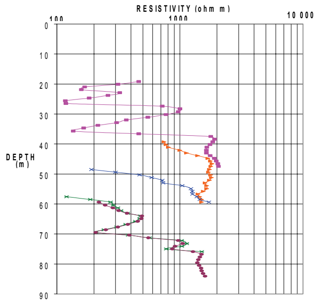
FIGURE 38e SECTION THROUGH BOREHOLES DRILLED TO STRIKE LINEAR CONDUCTIVE FEATURE DROEGE GROND 135 DISTRICT KENHARDT
