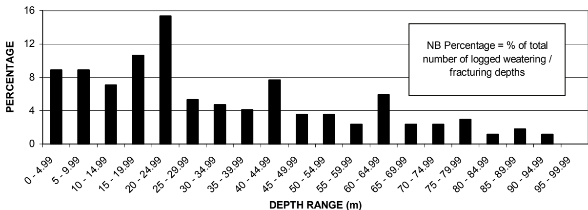
FIGURE 13e DISTRIBUTION OF LOGGED DEPTHS OF WEATHERING AND FRACTURING SUBDIVISION 5
