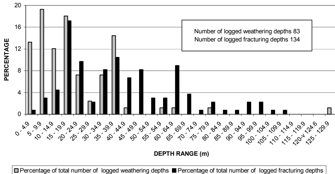
FIGURE 23d DISTRIBUTION OF LOGGED DEPTHS OF WEATHERING AND FRACTURING SUBDIVISION 18
