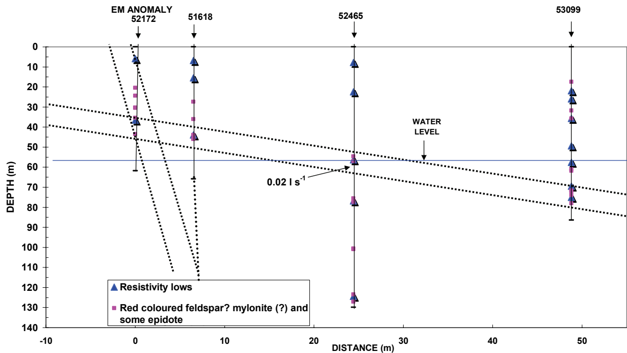
FIGURE 38e SECTION THROUGH BOREHOLES DRILLED TO STRIKE LINEAR CONDUCTIVE FEATURE DROEGE GROND 135 DISTRICT KENHARDT
