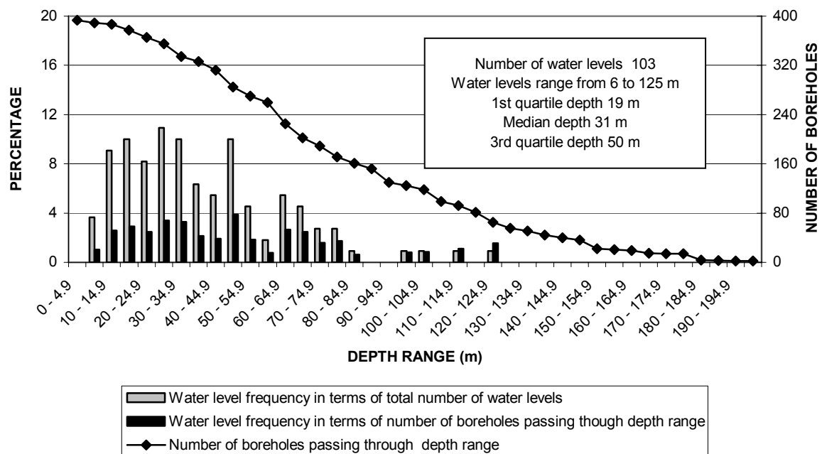
FIGURE 17b DISTRIBUTION OF WATER LEVELS SUBDIVISION 9
