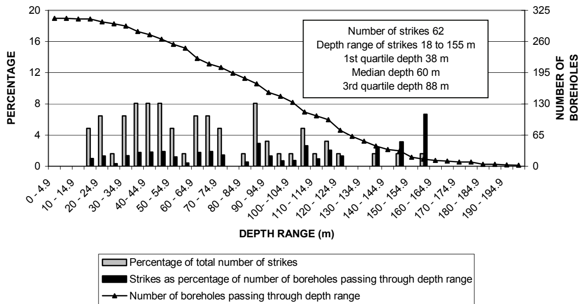
FIGURE 19c DISTRIBUTION OF STRIKES BELOW SURFACE SUBDIVISION 11
