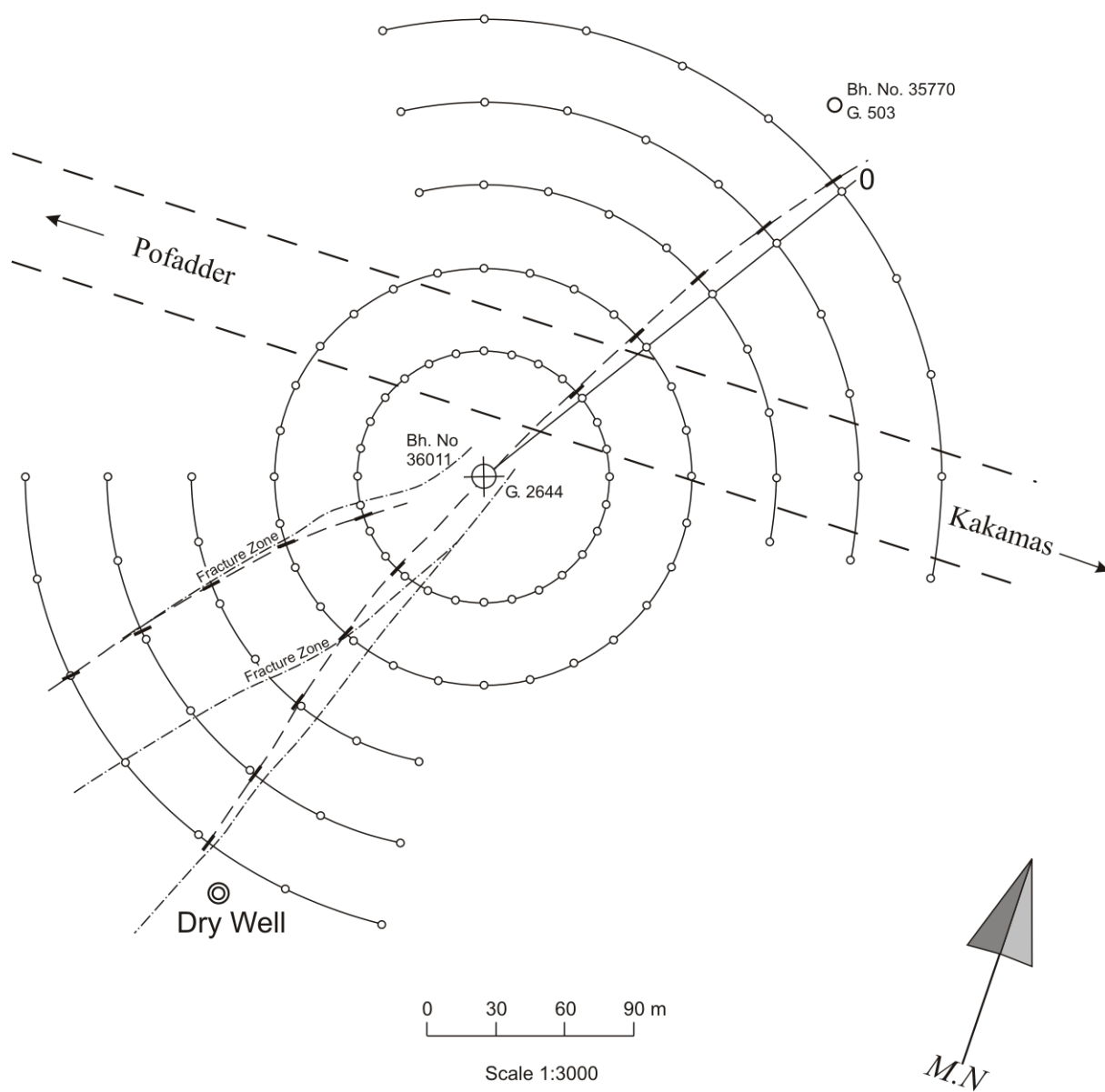
Figure 34a: Electromagnetic survey at sites G503 and G2644 (boreholes No's 35770 and 36011) Hellum 2 portion of Lucas Vlei 93 Kenhardt District
