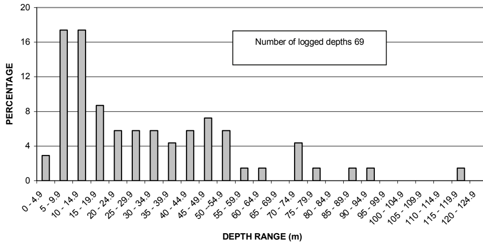
FIGURE 16d DISTRIBUTION OF LOGGED DEPTHS OF WEATHERING AND FRACTURING SUBDIVISION 8
