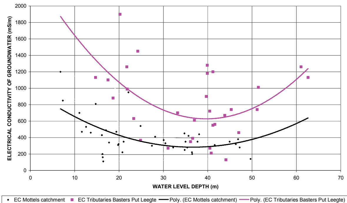
FIGURE 7 RELATIONSHIP BETWEEN PIEZOMETRIC LEVEL AND GROUNDWATER EC MOTTELS RIVER AND BASTERS PUT LEEGTE CATCHMENTS
