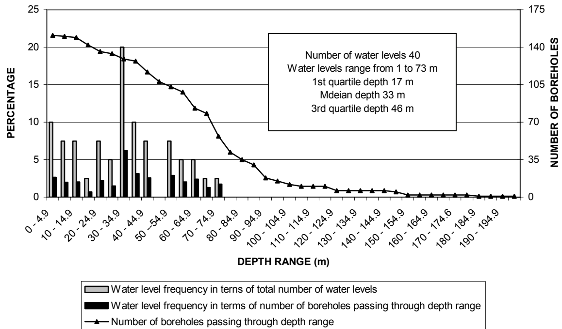
FIGURE 15b DISTRIBUTION OF WATER LEVELS SUBDIVISION 7
