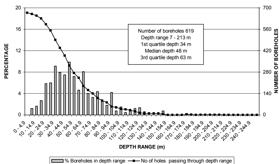
FIGURE12a DISTRIBUTION OF BOREHOLE DEPTHS SUBDIVISION 4
