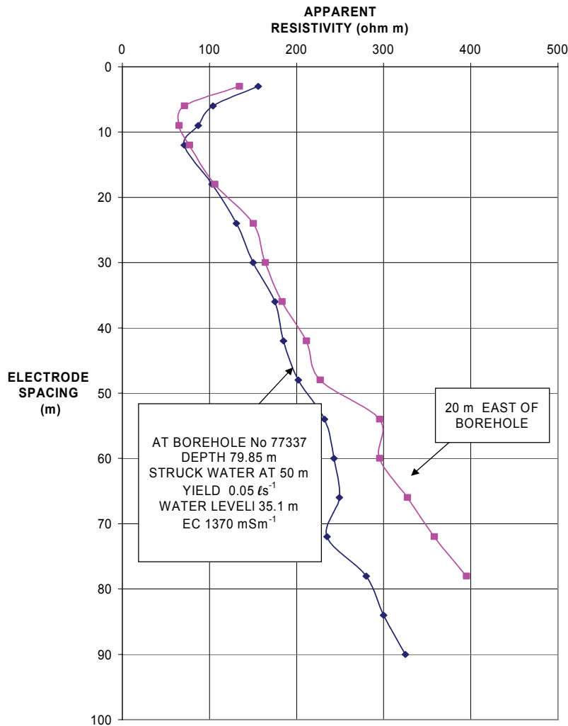
FIGURE 31 WENNER SOUNDINGS AT BOREHOLE No 77337 WITKOPJES 258 KENHARDT DISTRICT
