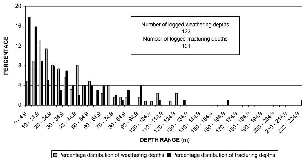
FIGURE 22f DISTRIBUTION OF DEPTHS OF WEATHERING AND DEPTHS OF FRACTURING SUBDIVISION 16
