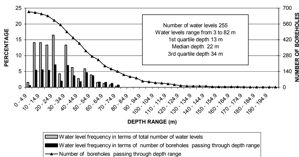
FIGURE12b DISTRIBUTION OF WATER LEVELS SUBDIVISION 4
