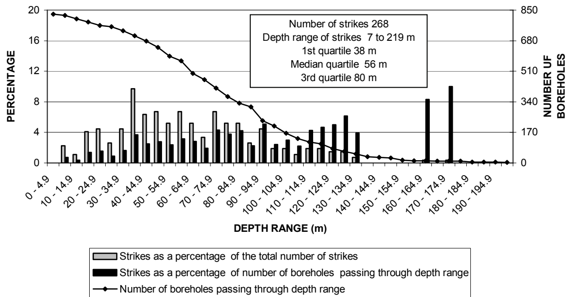
FIGURE 22c DISTRIBUTION OF STRIKES BELOW SURFACE SUBDIVISION 16
