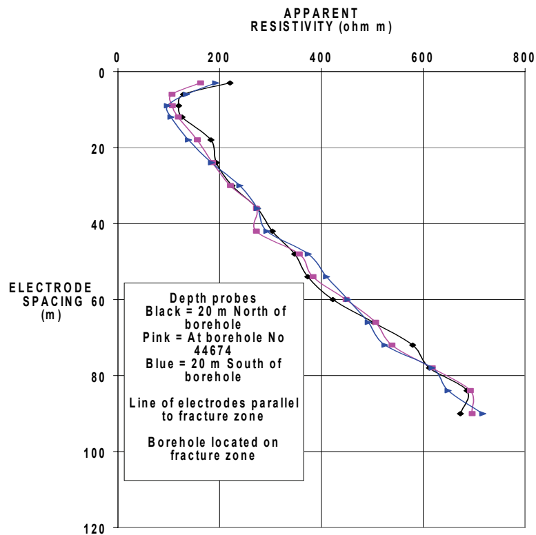
FIGURE 35c WENNER DEPTH PROBES AT BOREHOLE No 44674 HELLUM PT LUCAS VLEI 93
