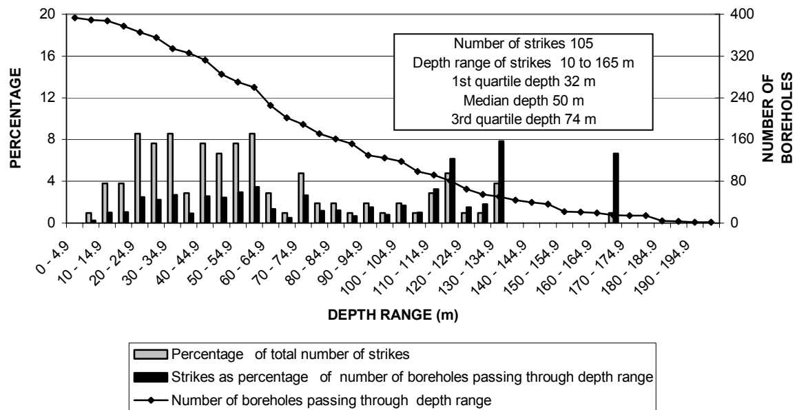
FIGURE 17c DISTRIBUTION OF STRIKES BELOW SURFACE SUBDIVISION 9
