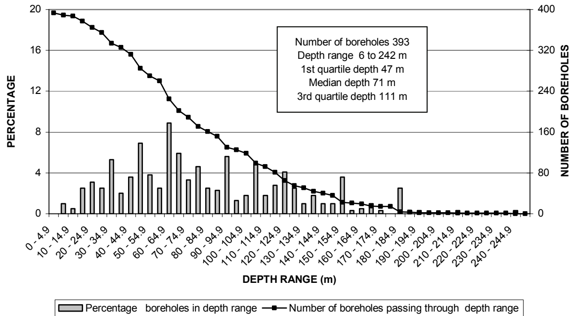
FIGURE17a DISTRIBUTION OF BOREHOLE DEPTHS SUBDIVISION 9
