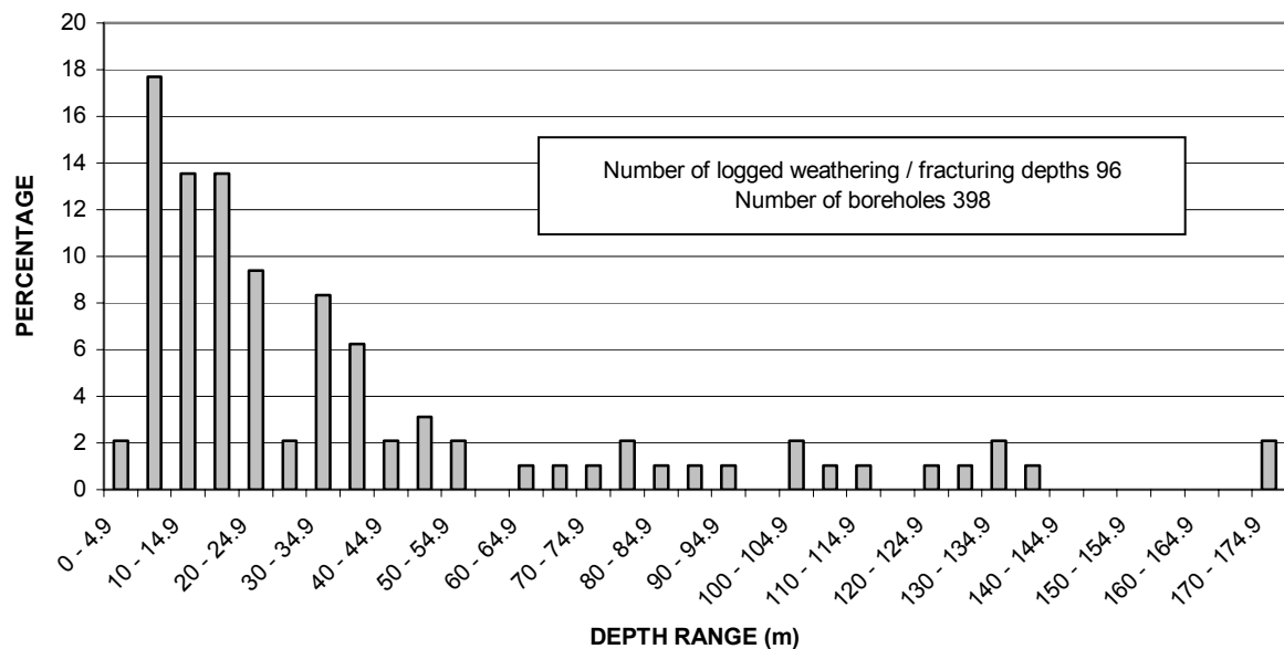
FIGURE 18d DISTRIBUTION OF LOGGED DEPTHS OF WEATHERING AND FRACTURING SUBDIVISION 10
