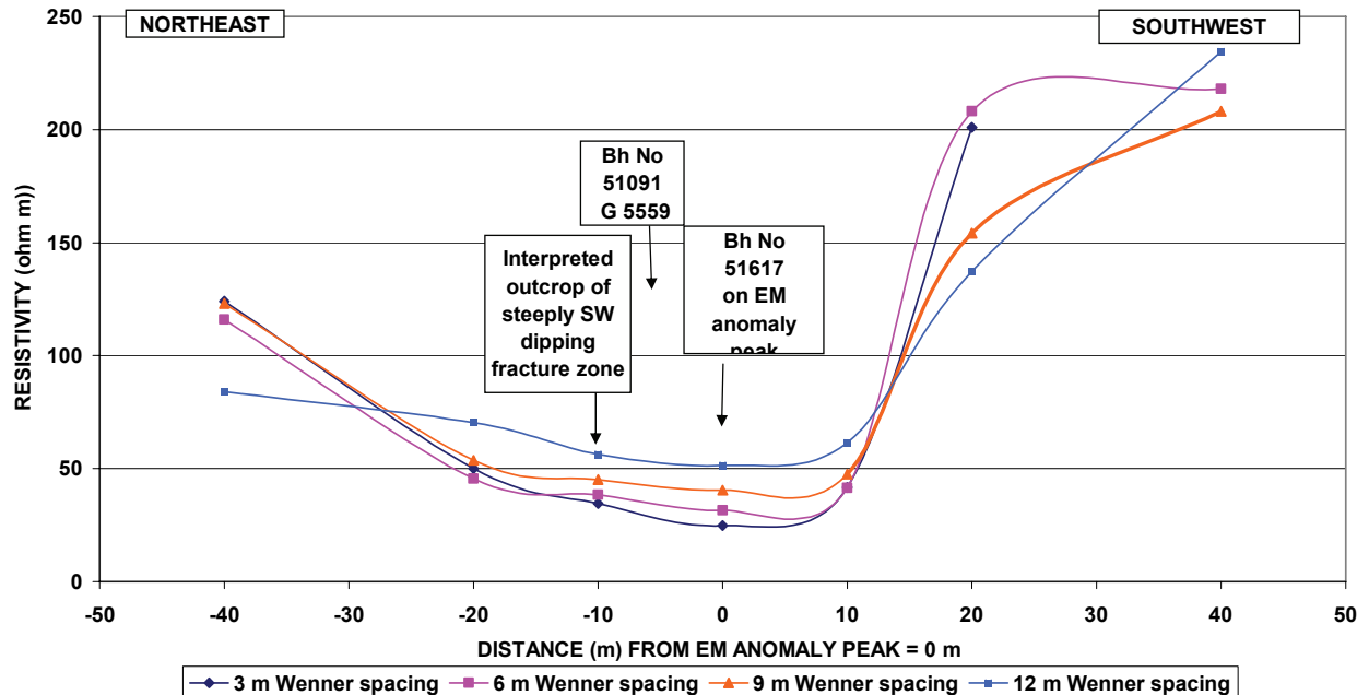
FIGURE 40c HORIZONTAL WENNER PROFILING ACROSS EM ANOMALY SWART OUP 80 KENHARDT DISTRICT
