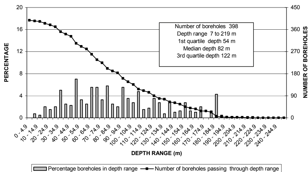
FIGURE18a DISTRIBUTION OF BOREHOLE DEPTHS SUBDIVISION 10
