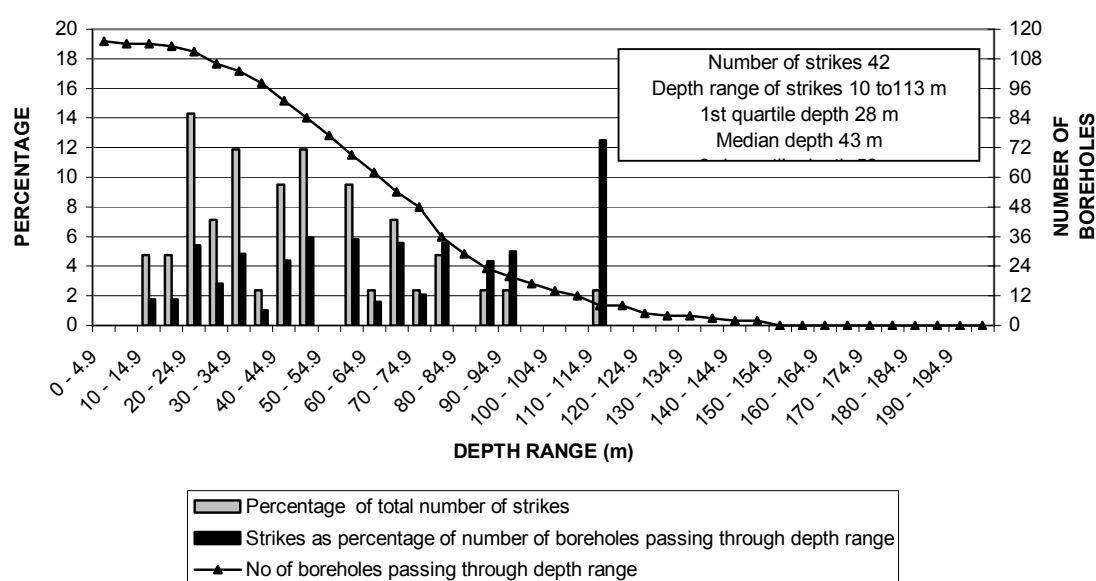
FIGURE 20c DISTRIBUTION OF STRIKES BELOW SURFACE SUBDIVISION 12
