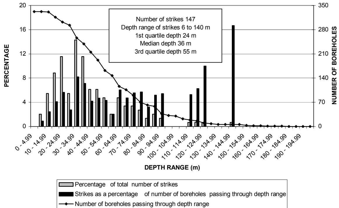
FIGURE 13c DISTRIBUTION OF STRIKES BELOW SURFACE SUBDIVISION 5
