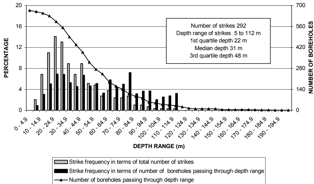
FIGURE 12c DISTRIBUTION OF STRIKES BELOW SURFACE SUBDIVISION 4
