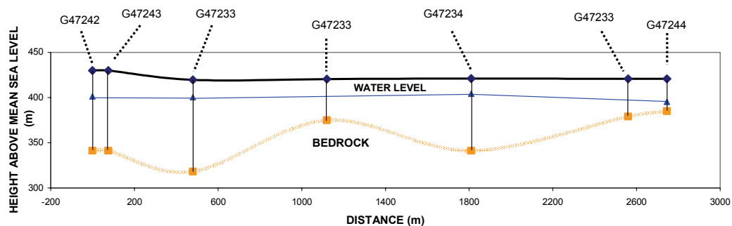
FIGURE 9 SECTION THROUGH CAINOZOIC DEPOSITS 3 km UPSTREAM FROM HENKRIES SPRING
