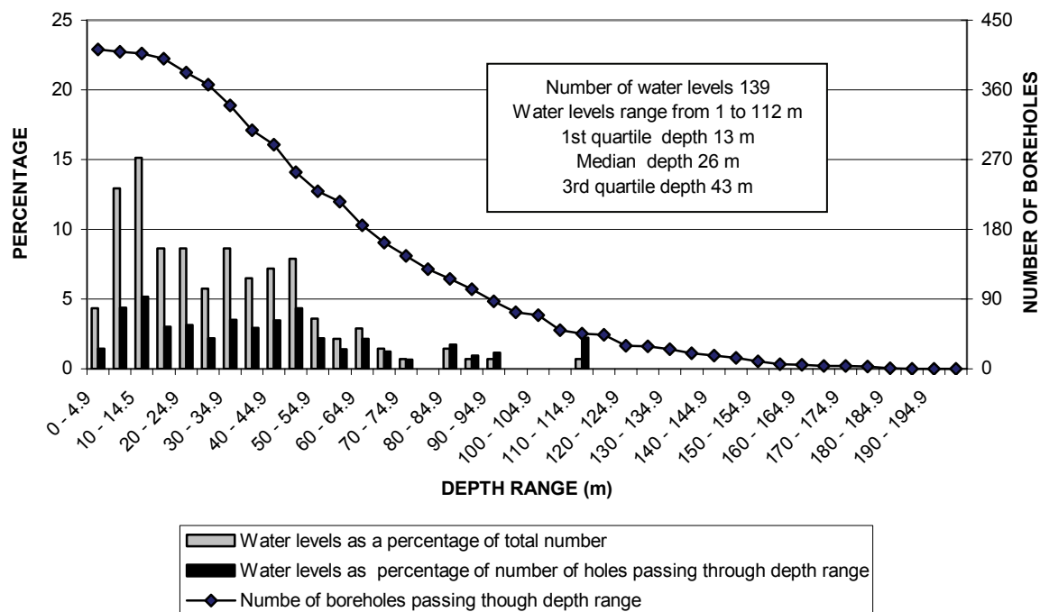
FIGURE14b DISTRIBUTION OF WATER LEVELS SUBDIVISION 6
