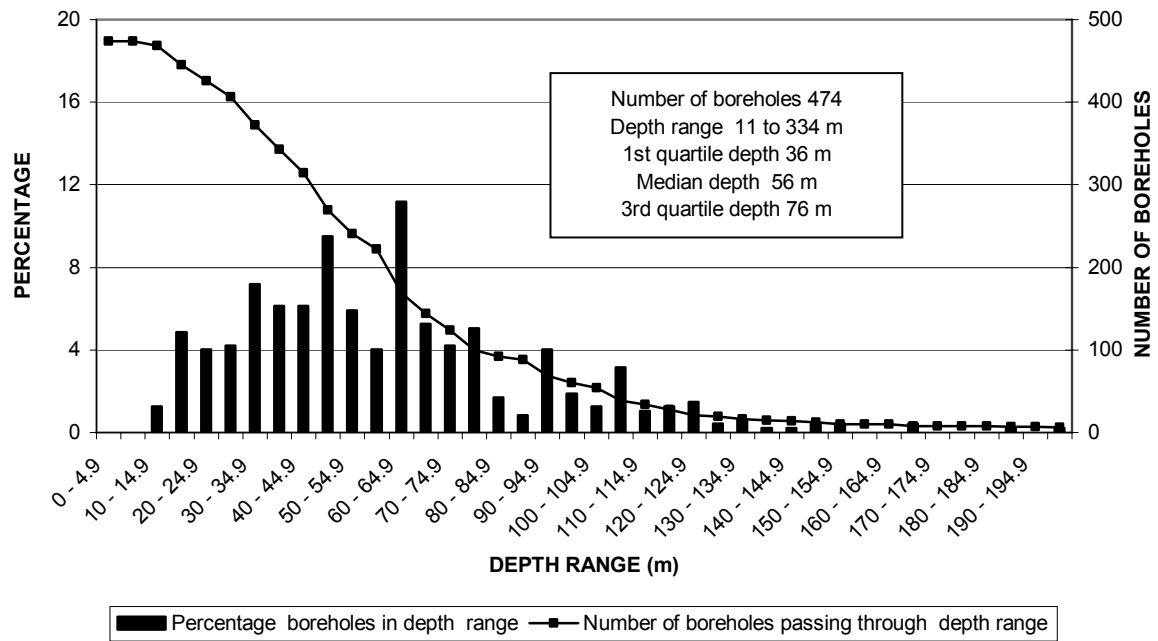
FIGURE 23a DISTRIBUTION OF BOREHOLE DEPTHS SUBDIVISION 18
