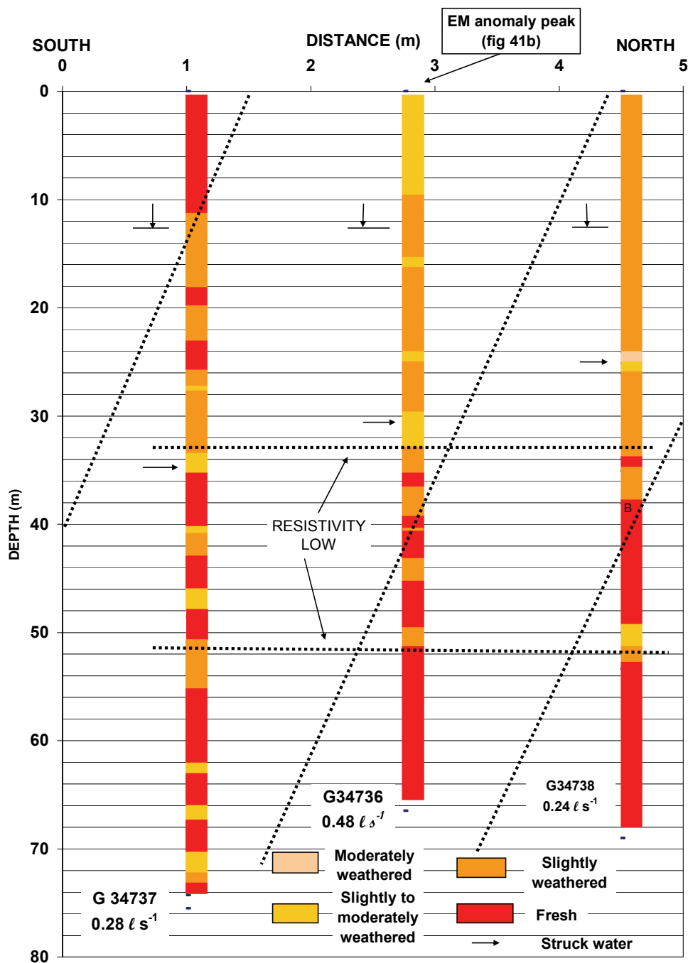
FIGURE 41j GEOLOGICAL SECTION THROUGH BOREHOLES G 34737, G34736 AND G34738 LOCALITY D, POFADDER
