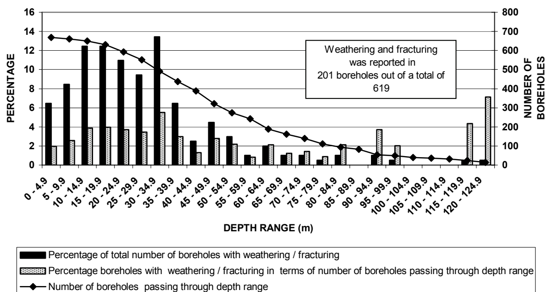
FIGURE 12g DISTRIBUTION OF LOGGED DEPTHS OF WEATHERING AND FRACTURING SUBDIVISION 4
