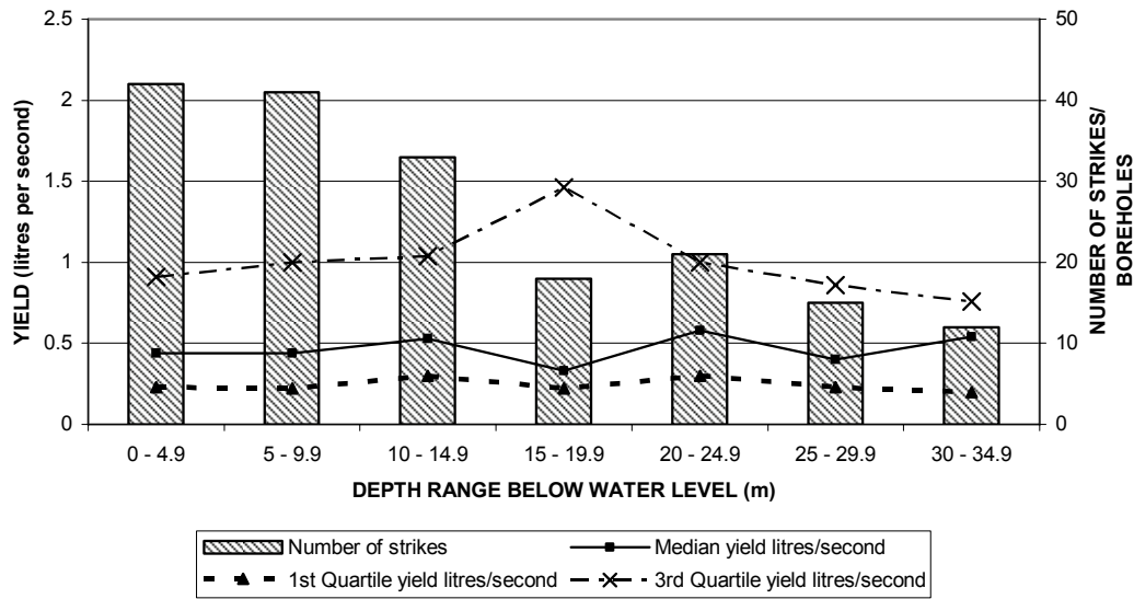
FIGURE 22e BOREHOLE YIELD VERSUS STRIKE DEPTH BELOW WATER LEVEL SUBDIVISION 16
