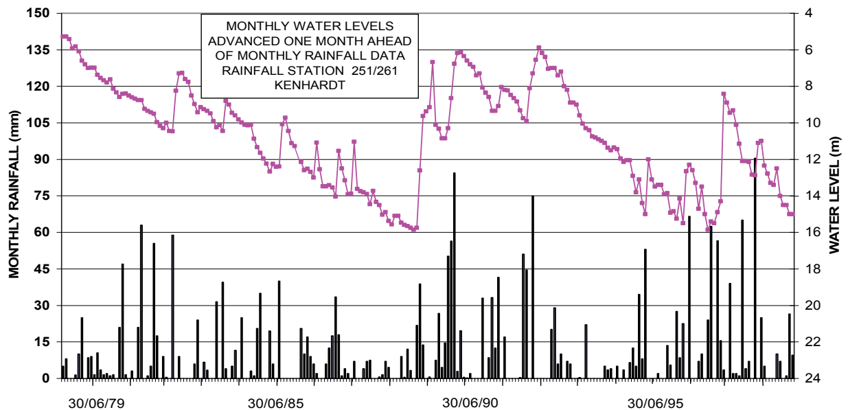
FIGURE 43 WATER LEVEL FLUCTUATION VALLEY OF DRIEKOP SE RIVIER KENHARDT (BOREHOLE G 27973)
