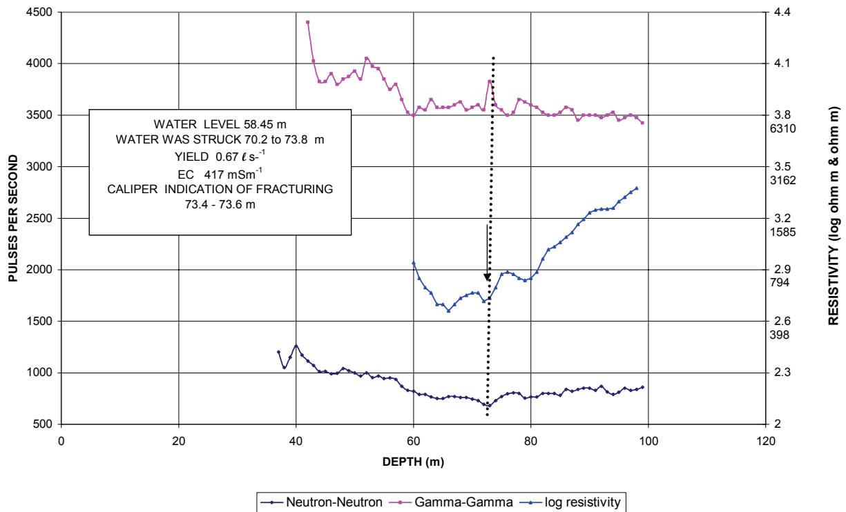
FIGURE 24 GAMMA-GAMMA, ELECTRICAL RESISTIVITY AND NEUTRON-NEUTRON LOGS OF BOREHOLE PBH 16 VAALPUTS
