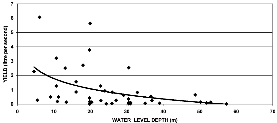
FIGURE 11 YIELD VERSUS WATER LEVEL SUBDIVISION 3
