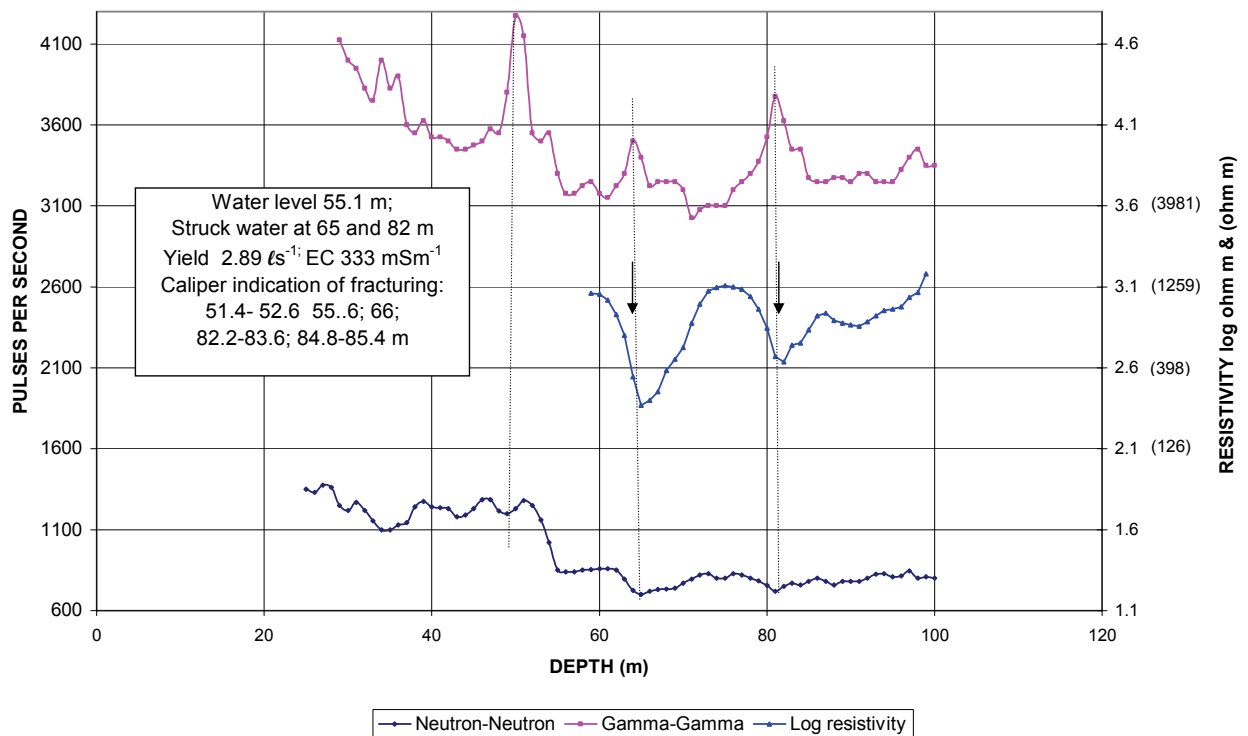
FIGURE 25 GAMMA-GAMMA, ELECTRICAL RESISTIVITY AND NEUTRON-NEUTRON LOGS BOREHOLE MON 4 VAALPUTS
