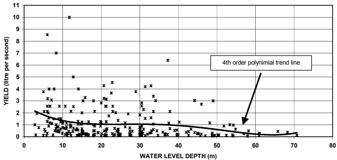
FIGURE 12e YIELD VERSUS WATER LEVEL SUBDIVISION 4
