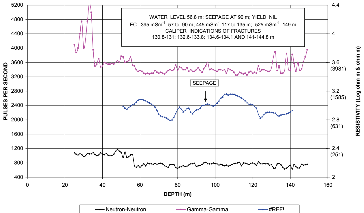
FIGURE 29 GAMMA-GAMMA, ELECTRICAL RESISTIVITY AND NEUTRON-NEUTRON LOGS OF BOREHOLE MON 14 VAALPUTS
