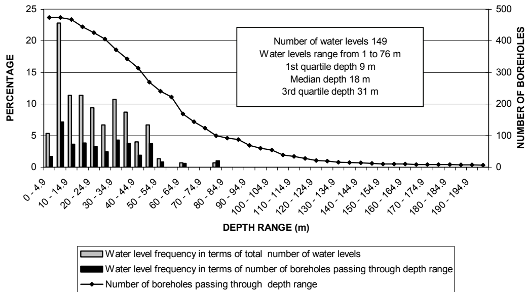
FIGURE 23b DISTRIBUTION OF WATER LEVELS SUBDIVISION 18
