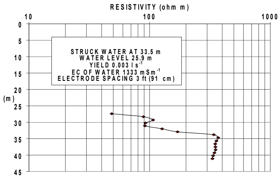
FIGURE 34c ELECTRICAL RESISTIVITY LOG OF BOREHOLE No 36011
