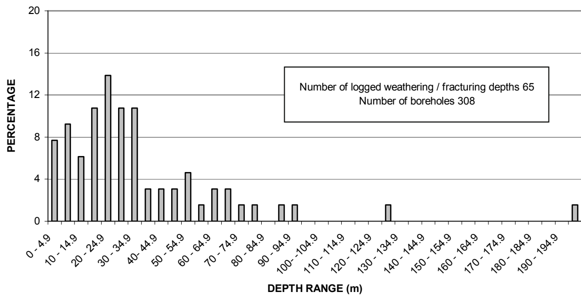
FIGURE 19d DISTRIBUTION OF LOGGED WEATHERING / FRACTURING DEPTHS SUBDIVISION 11
