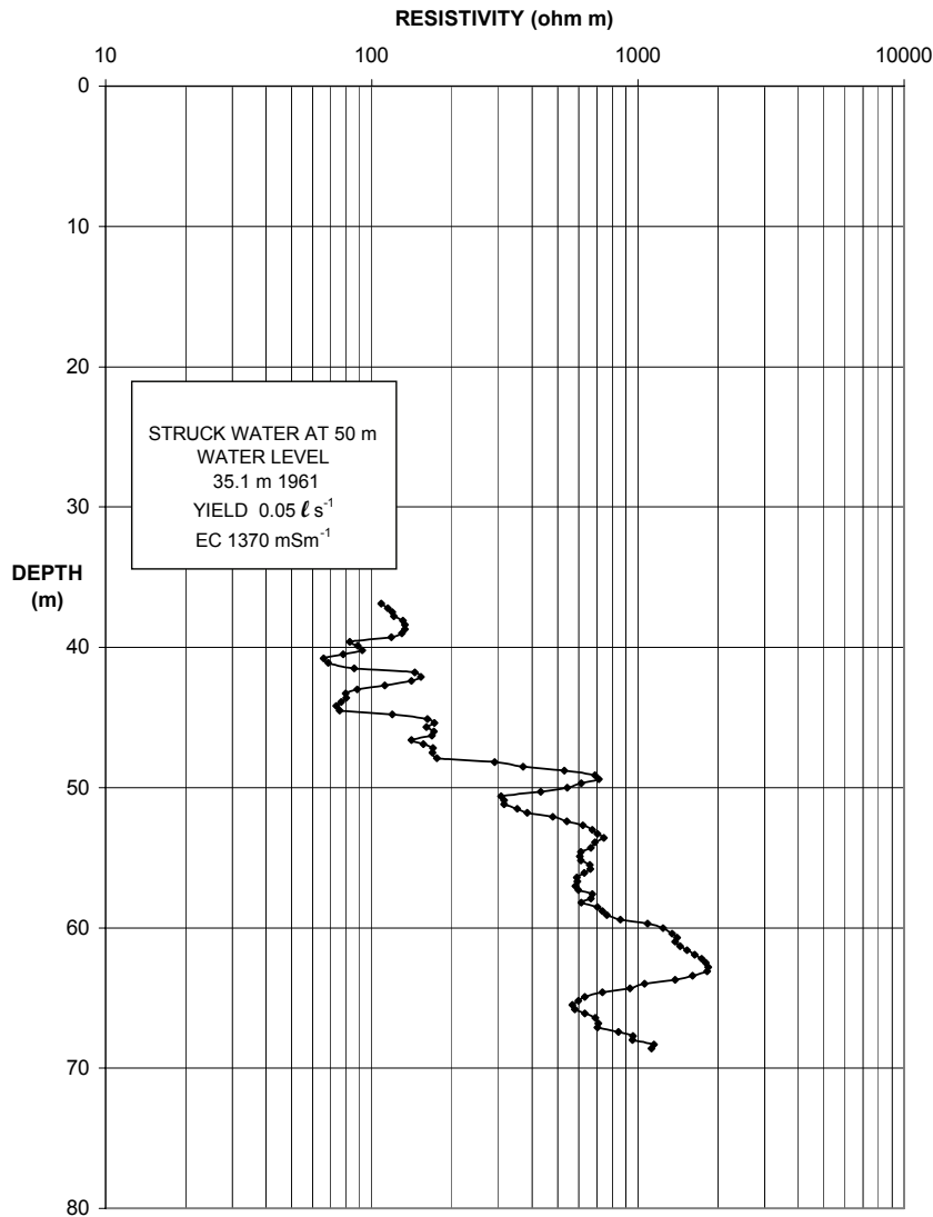
FIGURE 32 ELECTRICAL RESISTIVITY LOG OF BOREHOLE 77337 WITKOPJES 258 KENHARDT
