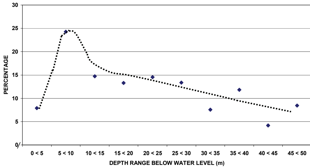
FIGURE 22d STRIKE FREQUENCY BELOW WATER LEVEL SUBDIVISION 18
