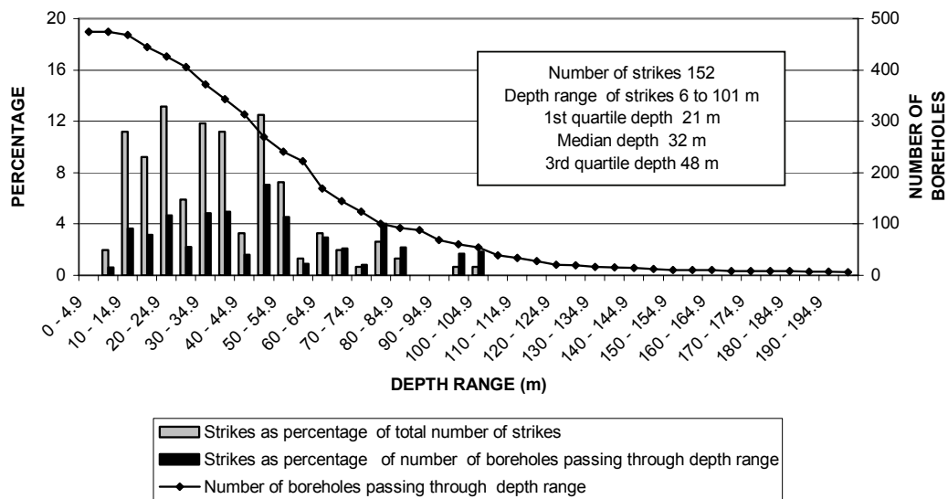
FIGURE 23c DISTRIBUTION OF STRIKES BELOW SURFACE SUBDIVISION 18
