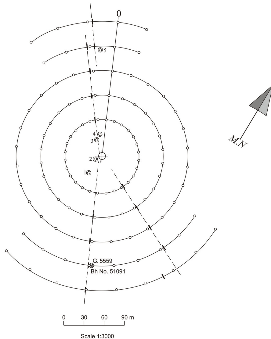
Figure 40a: Electromagnetic survey at borehole site G 5559 (Boreholes No's 51091 and 51616) Swart Oup 80 Kenhardt District
