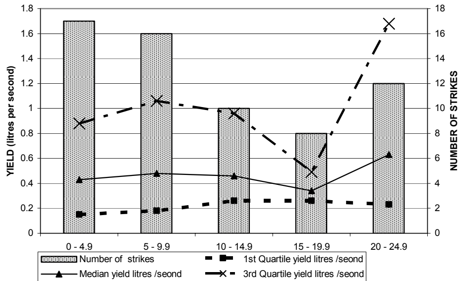
FIGURE 21d YIELD VERSUS STRIKE DEPTH BELOW WATER LEVEL SUBDIVISION 14 (HARD ROCK)
