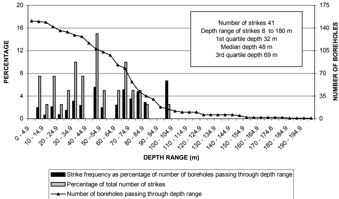
FIGURE15c DISTRIBUTION OF STRIKES BELOW SURFACE SUBDIVISION 7
