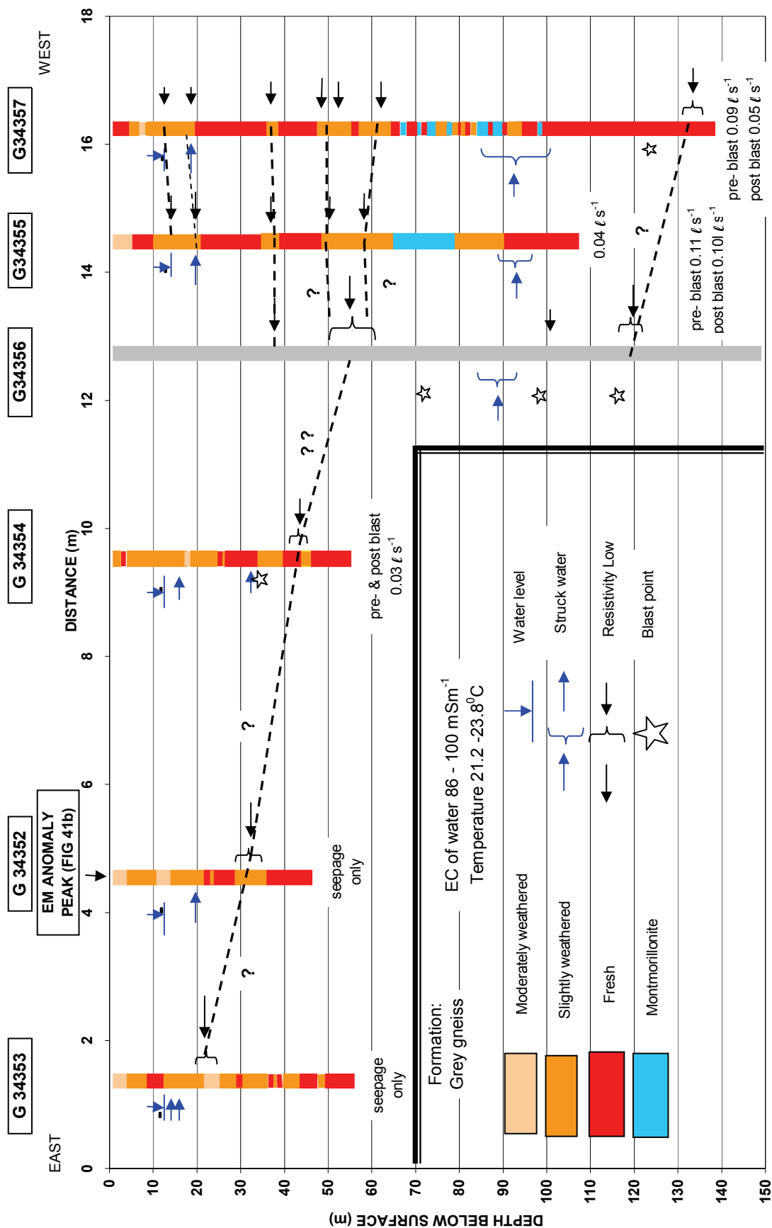
FIGURE 41f GEOLOGICAL SECTION THROUGH BOREHOLES No's G 34352 TO G 34357 ACROSS EM ANOMALY LOCALITY B POFADDER TOWN LANDS
