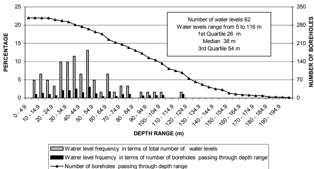
FIGURE 19b DISTRIBUTION OF WATER LEVELS SUBDIVISION 11
