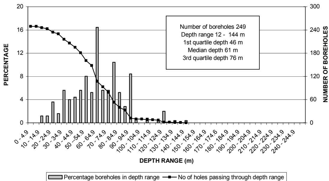
FIGURE16a DISTRIBUTION OF BOREHOLE DEPTHS SUBDIVISION 8
