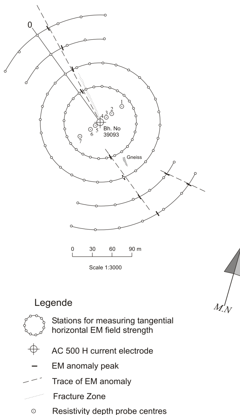
Figure 36a: Electromagnetic survey at site G2648 (borehole No 37093) Hellum 1 portion of Lucas Vlei 93 Kenhardt District
