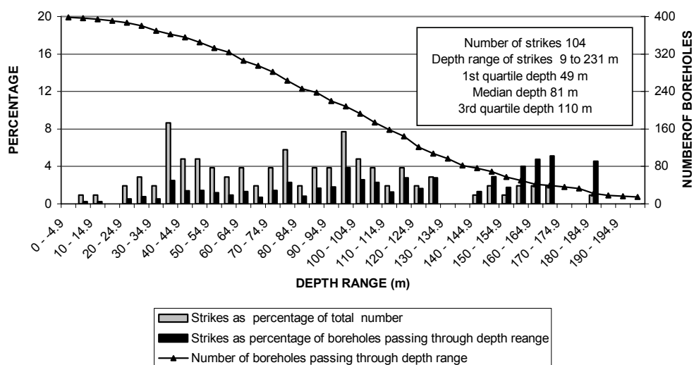
FIGURE 21c DISTRIBUTION OF STRIKES BELOW SURFACE SUBDIVISION 14
