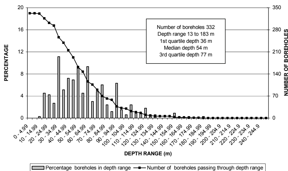
FIGURE 13a DISTRIBUTION OF BOREHOLE DEPTHS SUBDIVISION 5
