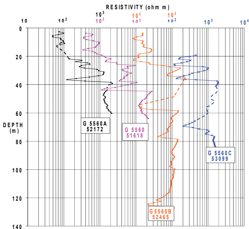
FIGURE 36c E.R. LOGS OF BOREHOLES ON AND OFF EM ANOMALY DROOGE GROND 135
