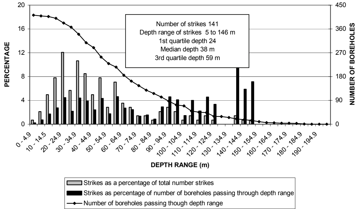
FIGURE 14c DISTRIBUTION OF STRIKES BELOW SURFACE SUBDIVISION 6
