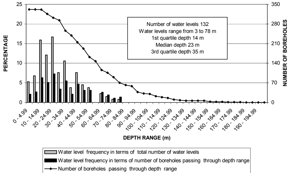
FIGURE13b DISTRIBUTION OF WATER LEVELS SUBDIVISION 5
