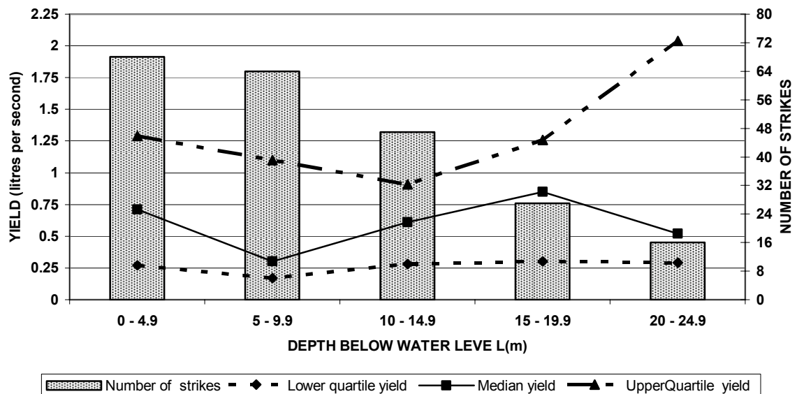
FIGURE 12f BOREHOLE YIELD VERSUS STRIKE DEPTH BELOW WATER LEVEL SUBDIVISION 4
