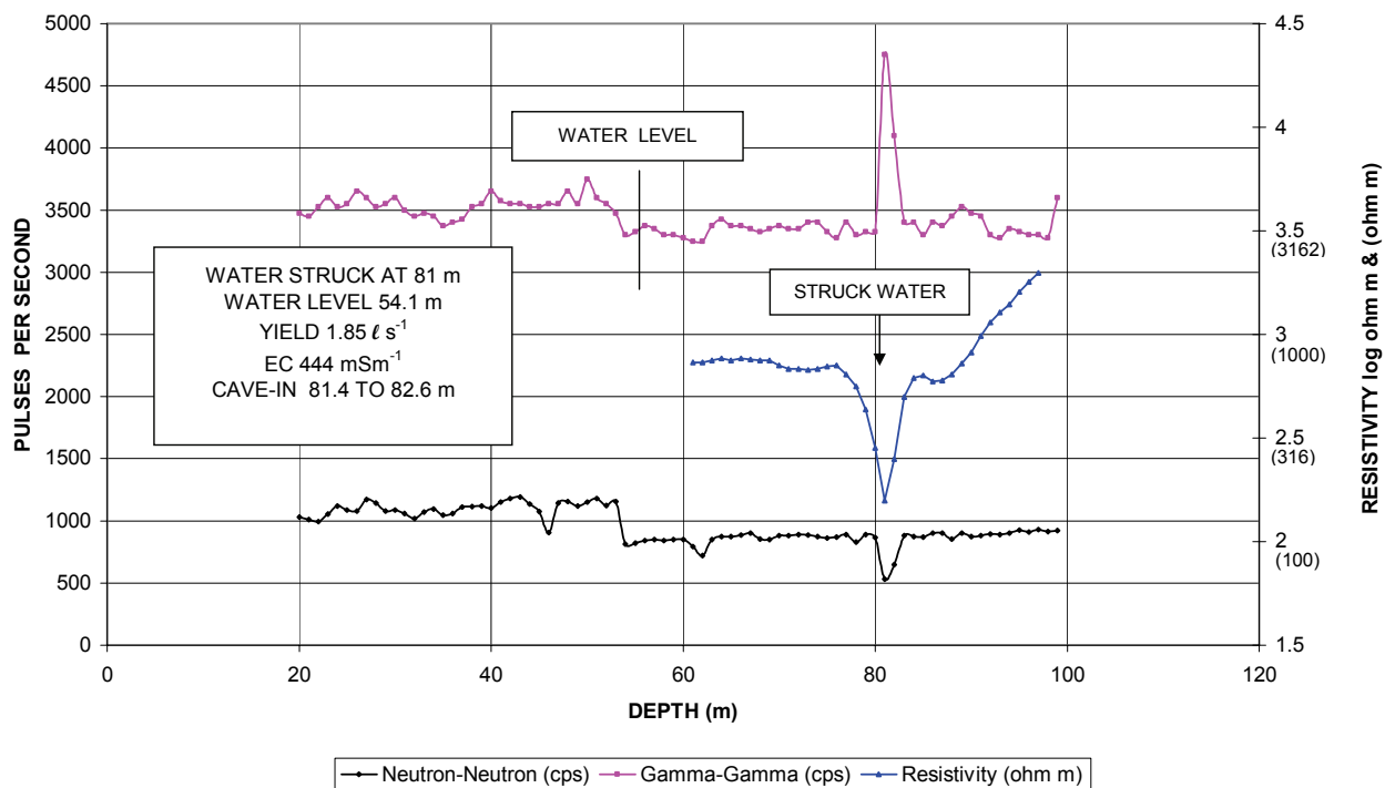
FIGURE 26 GAMMA-GAMMA, ELECTRICAL RESISTIVITY AND NEUTRON-NEUTRON LOGS OF BOREHOLE MON 11 VAALPUTS
