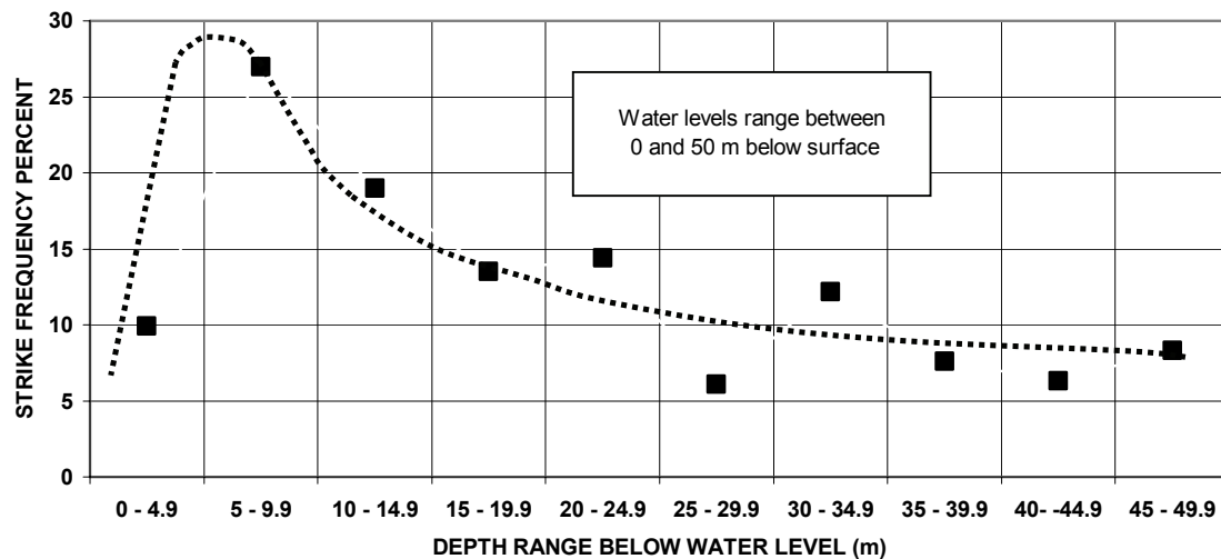
FIGURE 12d STRIKE FREQUENCY BELOW WATER LEVEL SUBDIVISION 4
