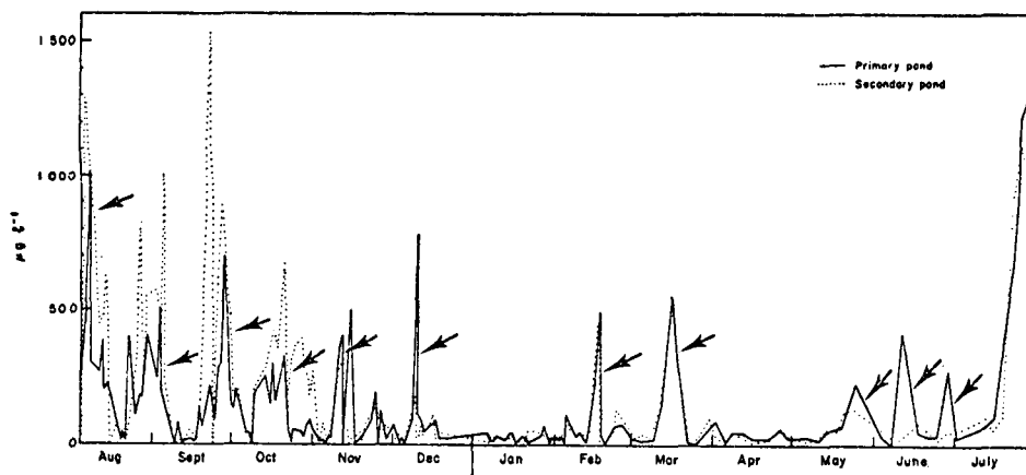
Figure 2 Chlorophyll a concentrations (in \mu\text{g l}^{-1} ) of pond system. Severe algal concentration declines are indicated by arrows.
