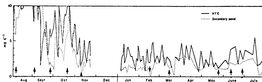
Figure 8 Ammonia-nitrogen concentrations (in mg \ell^{-1} ) of influent (HTE) and secondary pond. The arrows indicate the beginning of the noted algal concentration declines.
