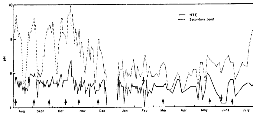
Figure 6 pH of influent (HTE) and secondary pond. The arrows indicate the beginning of the noted algal concentration declines.
