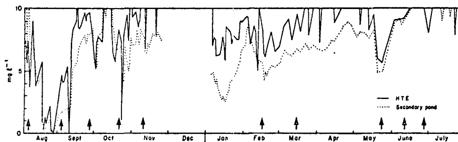
Figure 9 Nitrate-nitrogen concentrations (in \text{mg l}^{-1} ) of influent (HTE) and secondary pond. The arrows indicate the beginning of the noted algal concentration declines.
