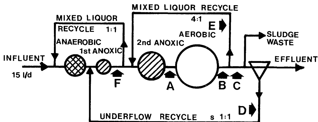
Figure 1 Configuration of modified UCT system for chlorination bulking control showing six possible chlorination dose points.
