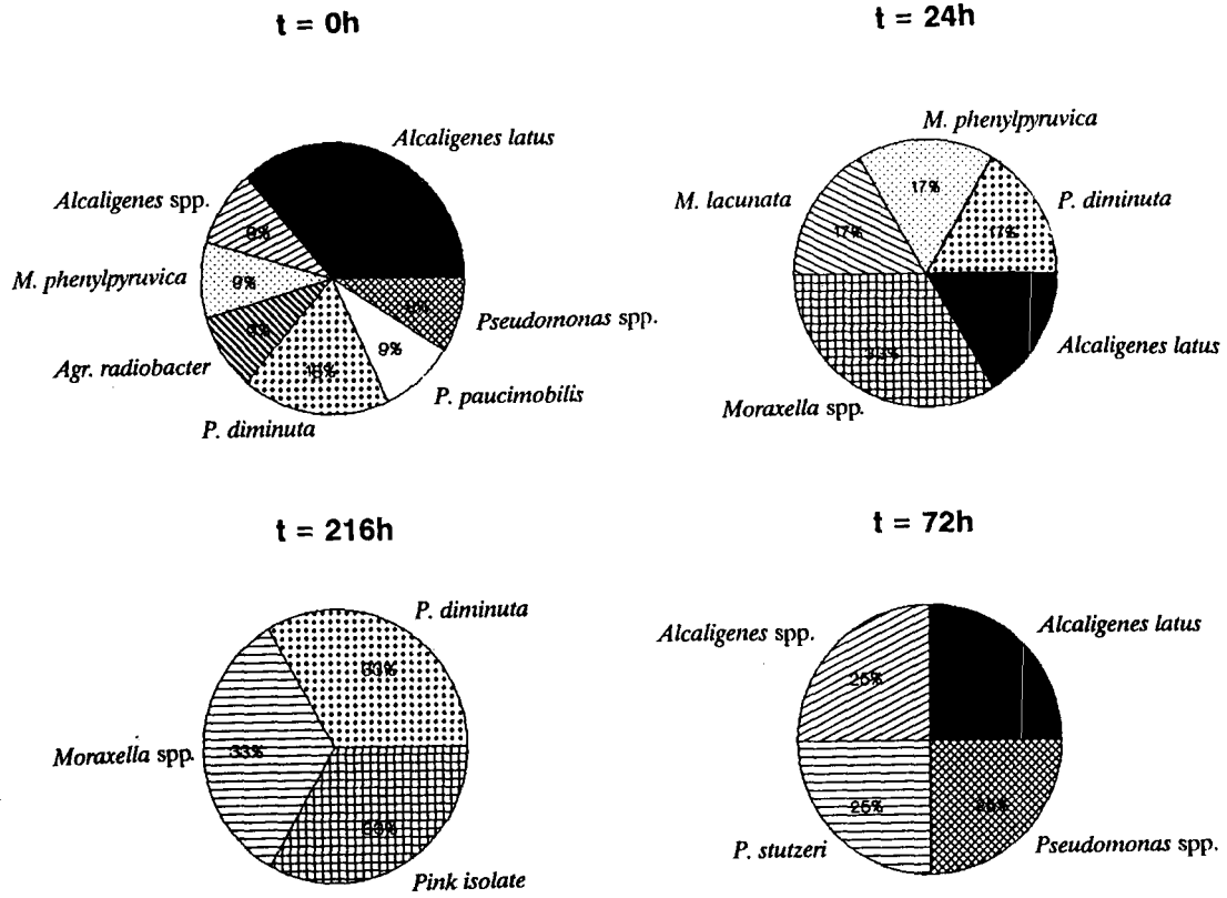
Figure 10 Community structure of tap-water sample as drawn (0 h) and after 24, 72 and 216 h storage at 20°C
