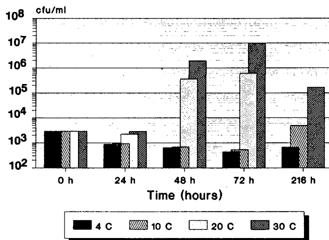
Figure 3 Total aerobic count of tap water sample stored at 4, 10, 20 and 30°C for 24, 48, 72 and 216 h (determined on R2A nutrient agar incubated at 30°C for 120 h). After 216 h the sample stored at 20°C was too numerous to count (TNTC)
