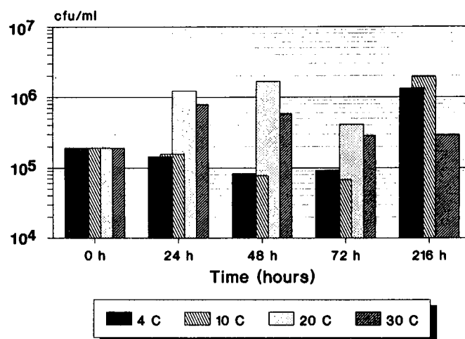
Figure 2 Total aerobic count of cooling-water sample stored at 4, 10, 20 and 30°C for 24, 48, 72 and 216 h (determined on R3A nutrient agar incubated at 30°C for 120 h). After 216 h the sample stored at 20°C was too numerous to count (TNTC)
