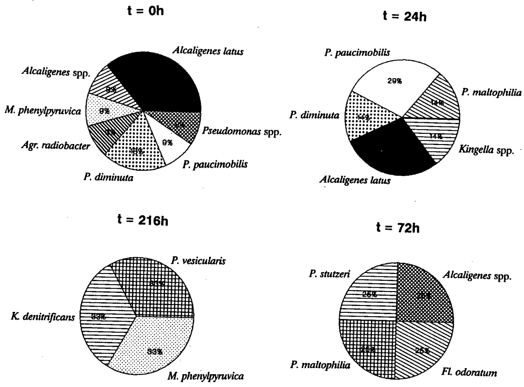
Figure 8 Community structure of tap-water sample as drawn (0 h) and after 24, 72 and 216 h storage at 4°C
