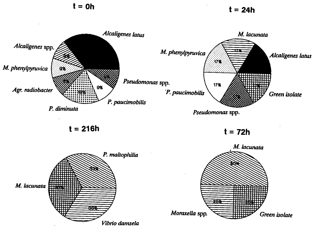
Figure 9 Community structure of tap-water sample as drawn (0 h) and after 24, 72 and 216 h storage at 10°C
