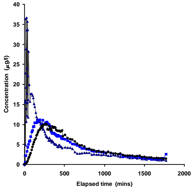
Figure 2 Residence distribution curves from the tracer study on 16 June 1997
