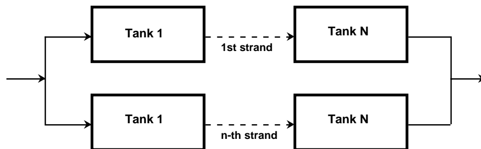
Figure 3 Schematic diagram showing the multi-strand concept of the Martin method
