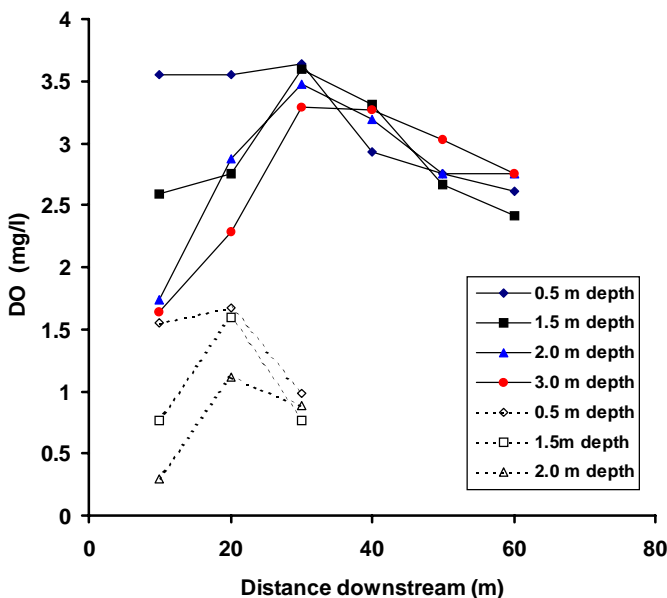
Figure 6 Dissolved oxygen concentrations downstream of aerator East-2 in May 1998 (dotted line) and downstream of aerator North in October 1998 (full line)
