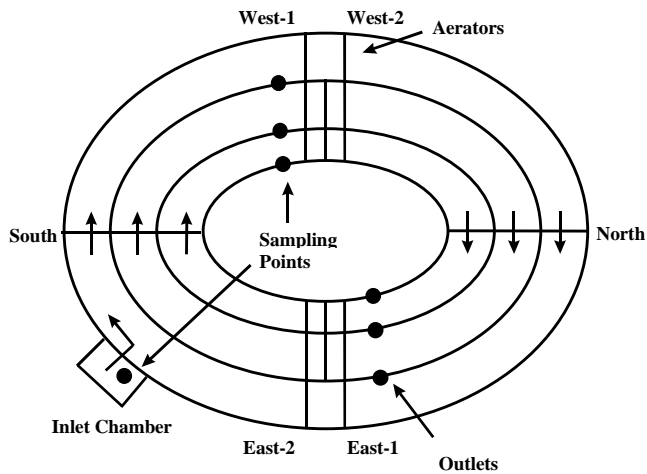
Figure 1 Schematic diagram of the Orbal system showing the sampling points
