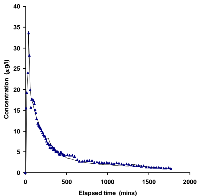
Figure 4 A comparison of the modelled tracer concentrations and the actual values obtained in the study on 16 June 1997
