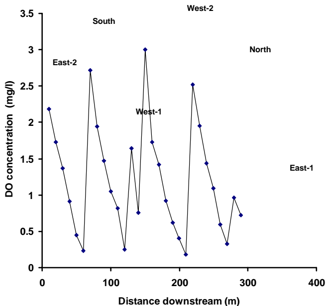
Figure 5 Dissolved oxygen survey in May 1998
