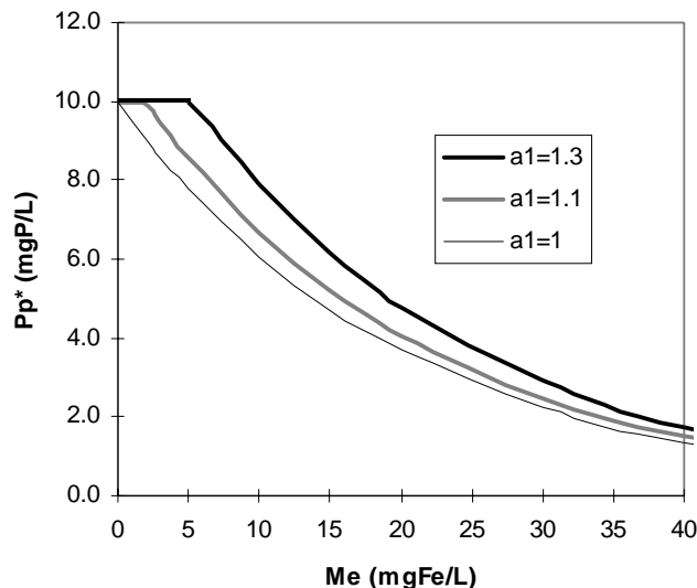
Figure 3 Theoretical effect of changing a_1 from 1 to 1.3 on P residual predicted from Eq. 13 for conditions in which P_{p0} = 10 mgP/l and a_2 = 0.5 for ferric chloride dosing, according to Briggs (1996). Note: a_1 and a_2 represent a_1 and a_2 in Fig. 3.
